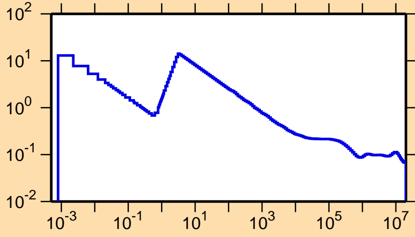
\sigma vs. E for ^{82}\text{Rb}(n,p)
