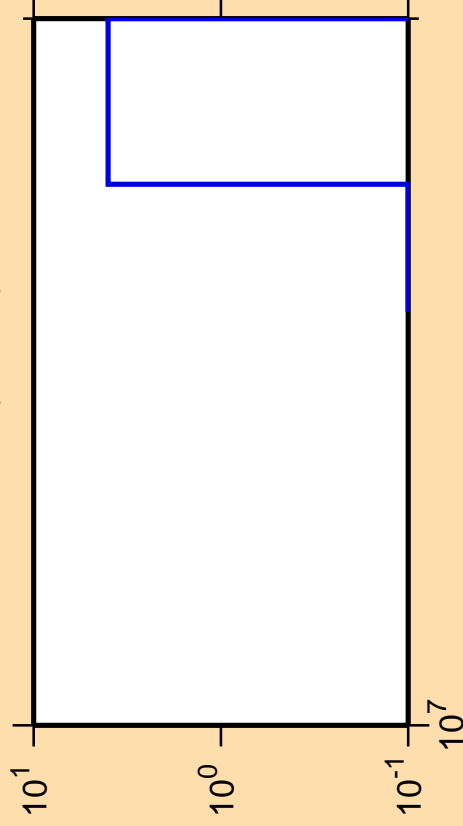
\Delta\sigma/\sigma vs. E for ^{82}\text{Rb} (mt 34)
