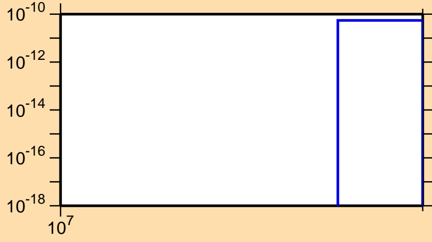
\sigma vs. E for ^{82}\text{Rb}(n,\text{pt})
