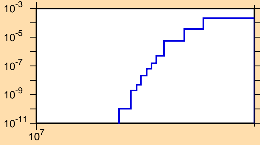
\sigma vs. E for ^{82}\text{Rb}(n,nd)
