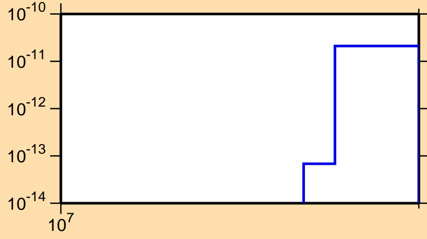
\sigma vs. E for ^{82}\text{Rb} (mt117)
