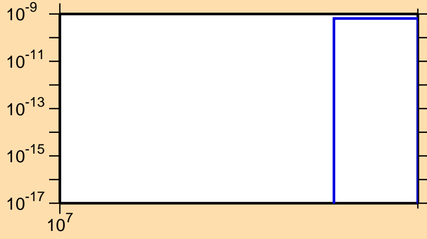
\sigma vs. E for ^{82}\text{Rb}(n,nt)
