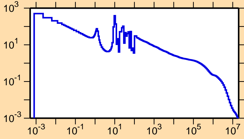
\sigma vs. E for ^{82}\text{Rb}(n,\gamma)
