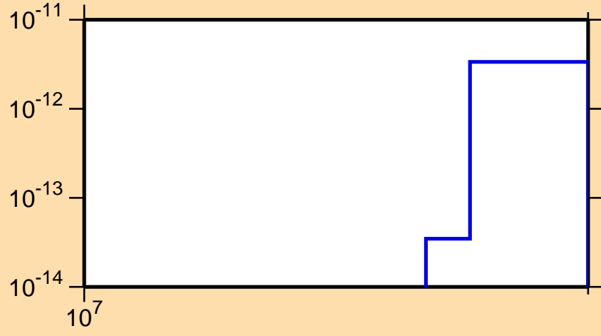
\sigma vs. E for ^{83}\text{Rb} (mt117)
