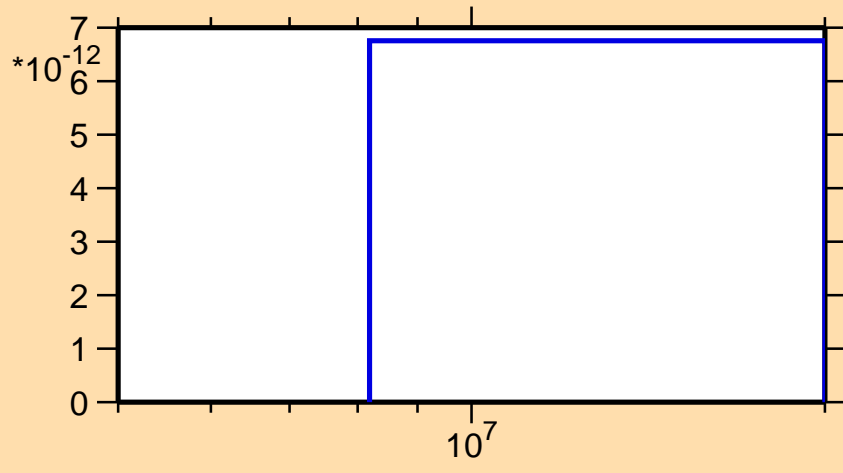
\sigma vs. E for ^{83}\text{Rb}(n,3n)
