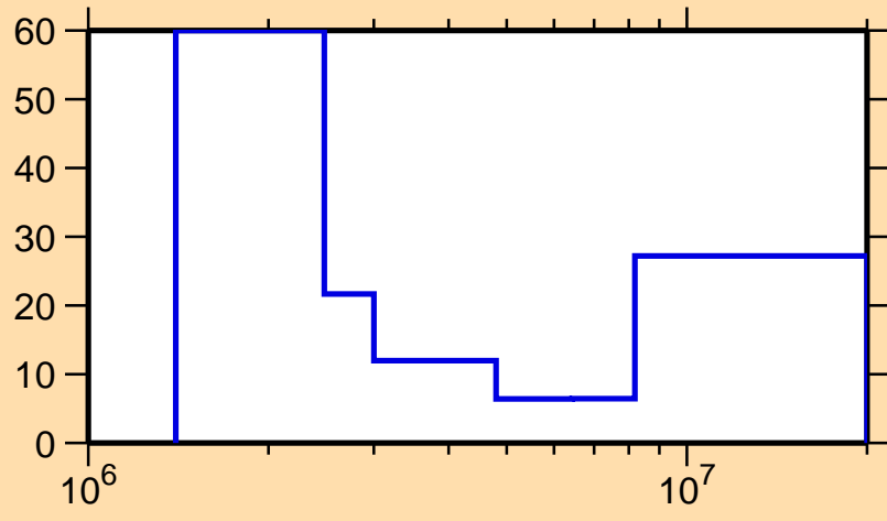
\Delta\sigma/\sigma vs. E for ^{83}\text{Rb}(n,n\text{cont.})
