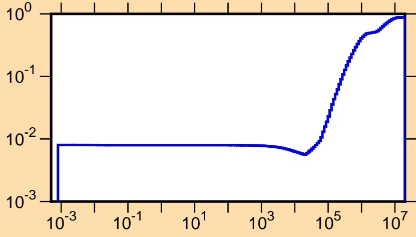
\mu vs. E for ^{84}\text{Rb}(\text{mt251})
