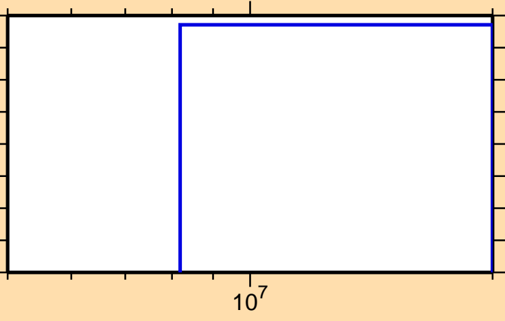
\sigma vs. E for ^{84}\text{Rb}(n,p\alpha)
