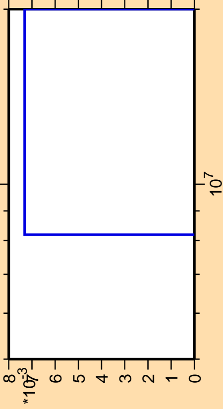
\Delta\sigma/\sigma vs. E for ^{84}\text{Rb}(n,\text{pd})
