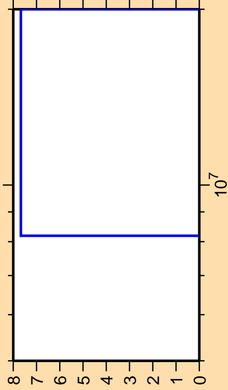
\Delta\sigma/\sigma vs. E for ^{84}\text{Rb}(n,3n)
