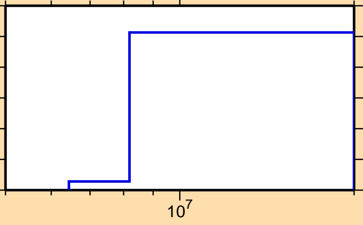
\sigma vs. E for ^{84}\text{Rb}(n,np)
