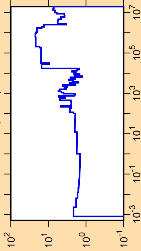
\Delta\sigma/\sigma vs. E for ^{85}\text{Rb}(n,\text{tot.})
