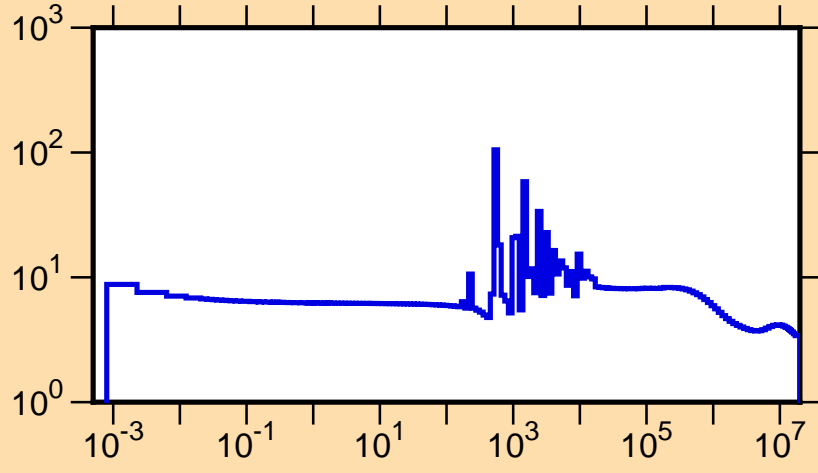
\sigma vs. E for ^{85}\text{Rb}(n,\text{tot.})
