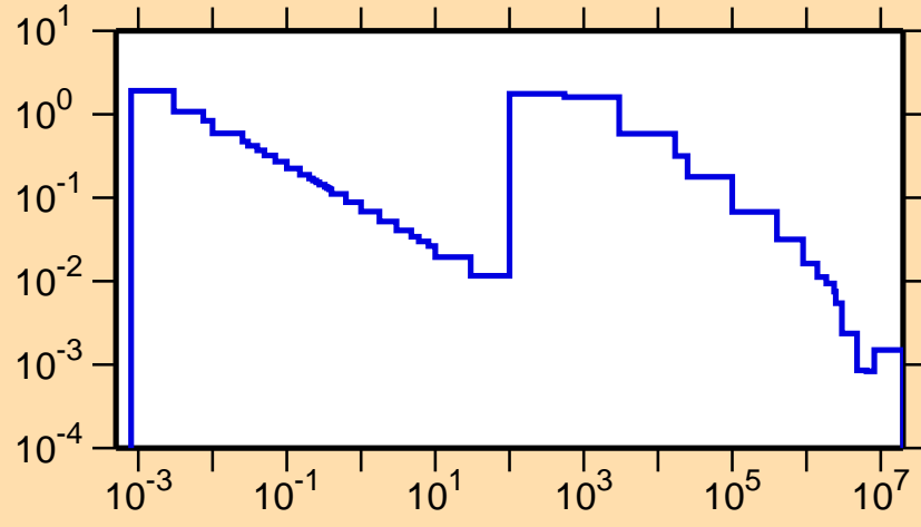
\sigma vs. E for ^{85}\text{Rb}(n,\gamma)
