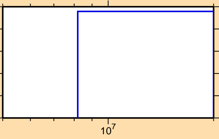
\sigma vs. E for ^{85}\text{Rb}(n,\text{nd})
