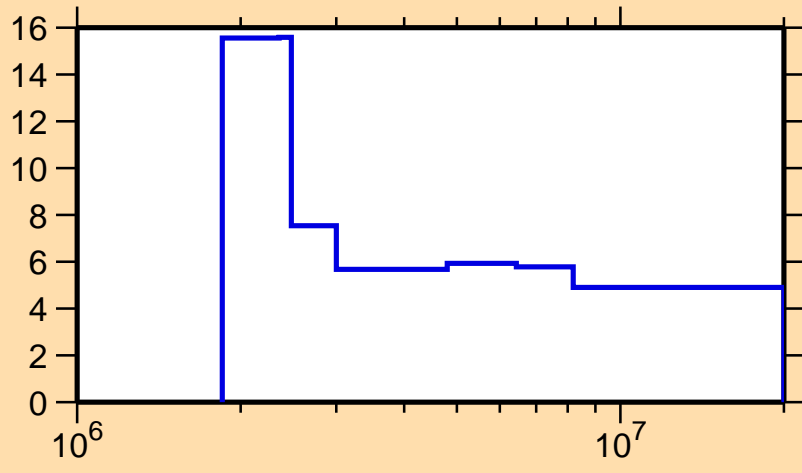
\Delta\sigma/\sigma vs. E for ^{85}\text{Rb}(n,n\text{onel.})
