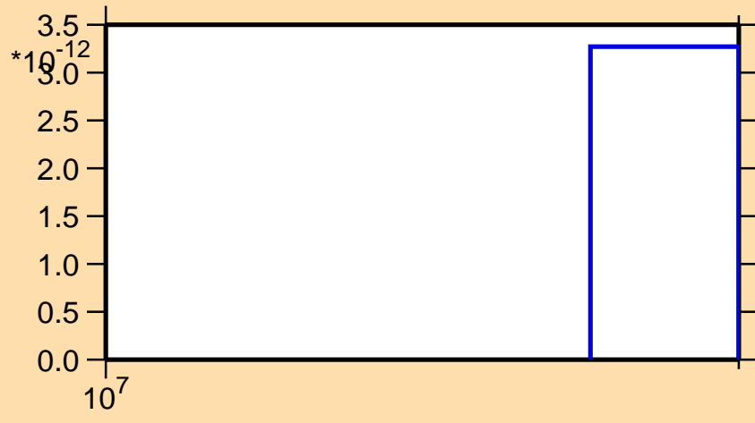
\sigma vs. E for ^{86}\text{Rb}(n,nt)
