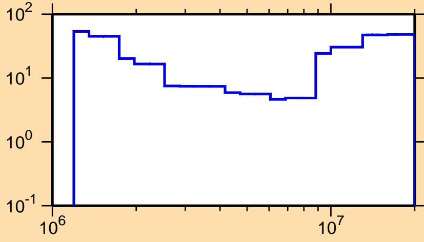
\Delta\sigma/\sigma vs. E for ^{86}\text{Rb}(n,n\text{cont.})
