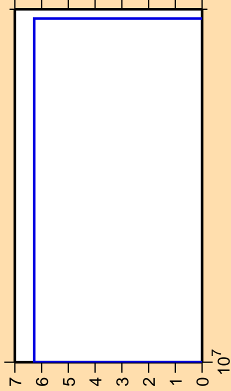
\Delta\sigma/\sigma vs. E for ^{86}\text{Rb}(n,\text{He}3)
