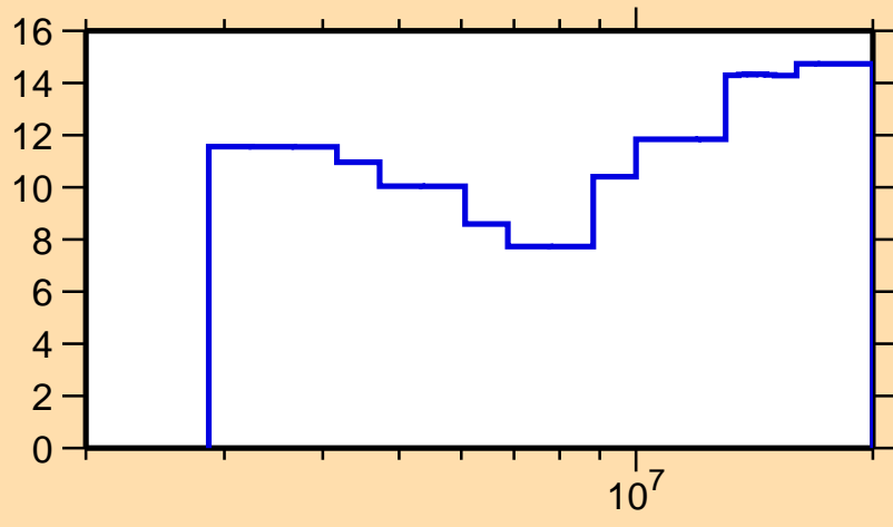
\Delta\sigma/\sigma vs. E for ^{87}\text{Rb}(n,el.)
