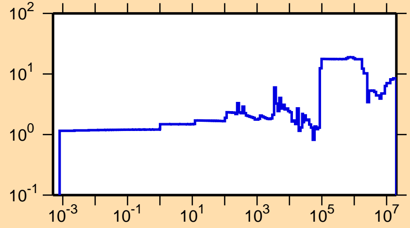
\Delta\sigma/\sigma vs. E for ^{87}\text{Rb}(n,\text{tot.})
