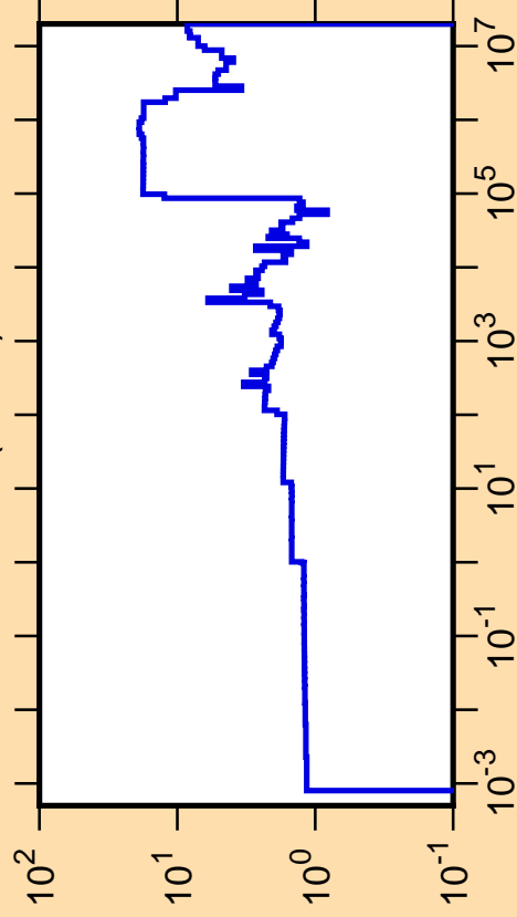
\Delta\sigma/\sigma vs. E for ^{87}\text{Rb}(n,\text{tot.})
