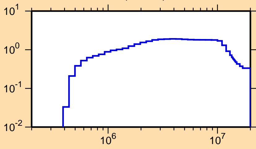
\sigma vs. E for ^{87}\text{Rb}(n,\text{inel.})
