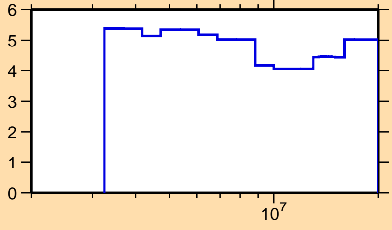
\Delta\sigma/\sigma vs. E for ^{87}\text{Rb}(n,n\text{nonel.})
