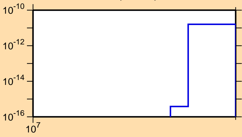
\sigma vs. E for ^{87}\text{Rb}(n,\text{He}3)
