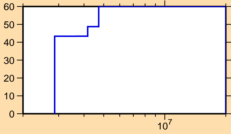
\Delta\sigma/\sigma vs. E for ^{87}\text{Rb}(n,\gamma)
