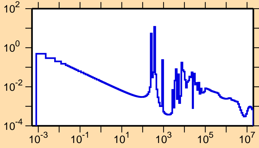
\sigma vs. E for ^{87}\text{Rb}(n,\gamma)
