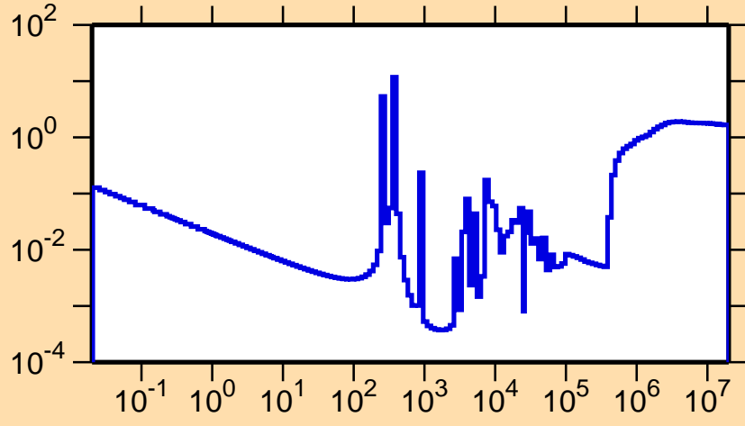
\sigma vs. E for ^{87}\text{Rb}(n,\text{nonel.})
