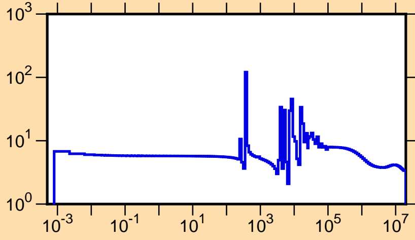
\sigma vs. E for ^{87}\text{Rb}(n,\text{tot.})
