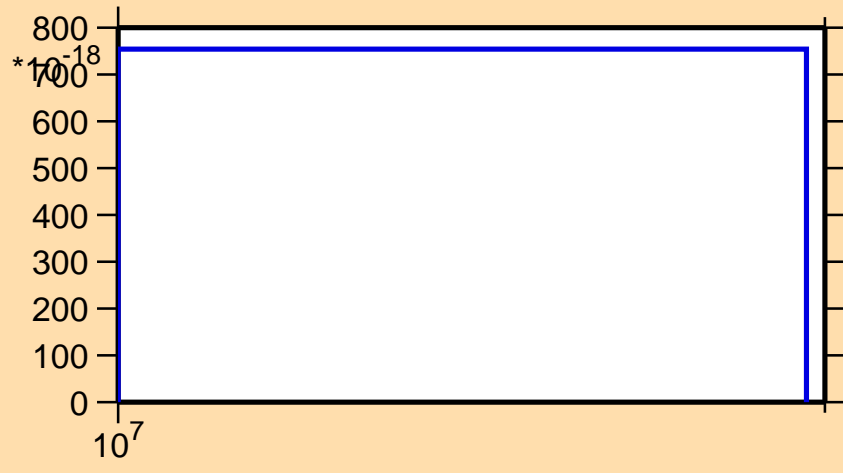
\sigma vs. E for ^{87}\text{Rb}(n,p\alpha)
