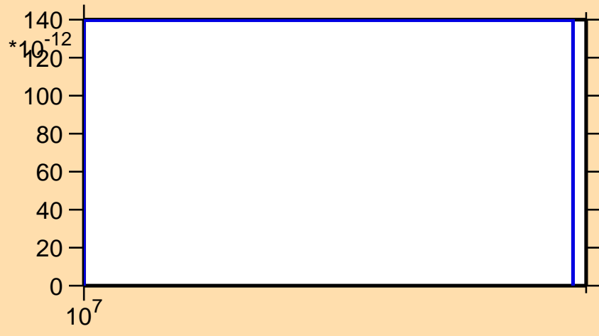
\sigma vs. E for ^{87}\text{Rb}(n,nd)
