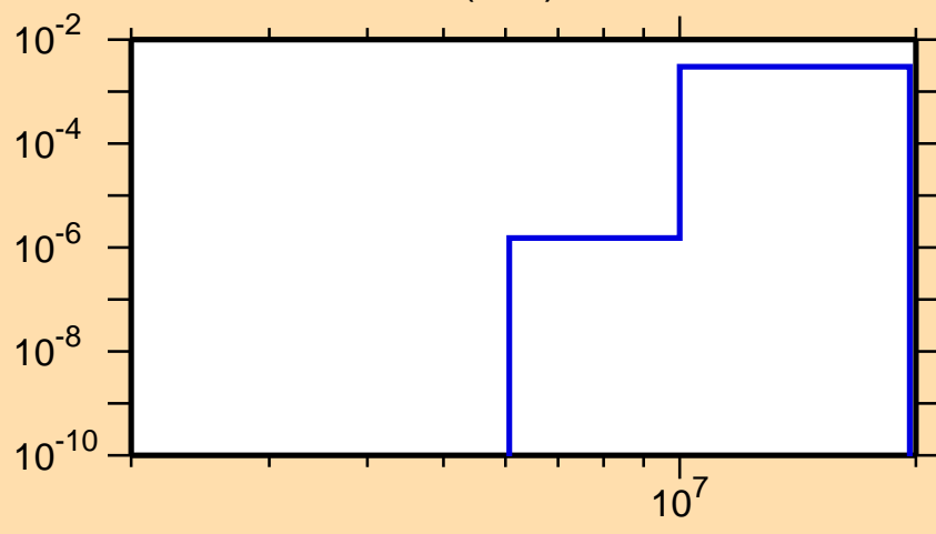
\sigma vs. E for ^{87}\text{Rb}(n,\alpha)
