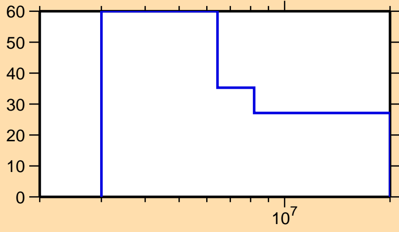
\Delta\sigma/\sigma vs. E for ^{87}\text{Rb}(n,p)
