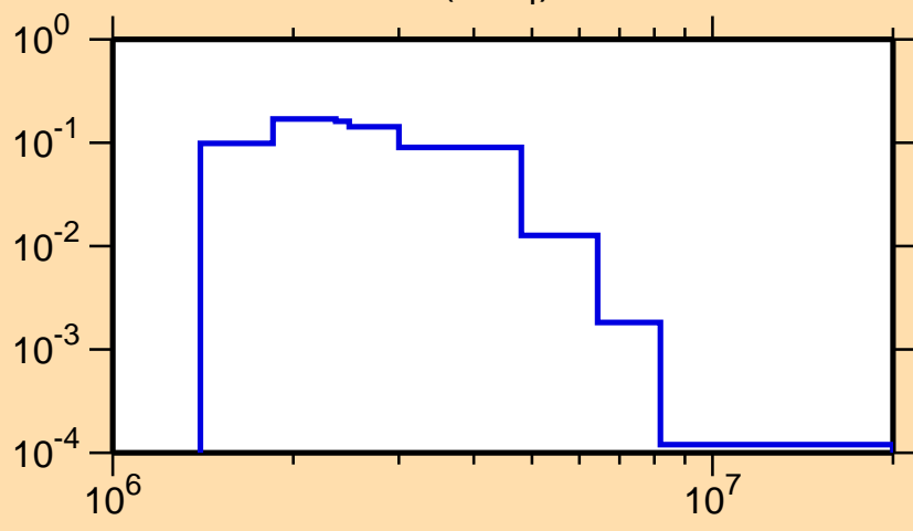
\sigma vs. E for ^{87}\text{Rb}(n,n_4)
