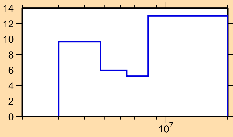
\Delta\sigma/\sigma vs. E for ^{87}\text{Rb}(n,n\text{cont.})
