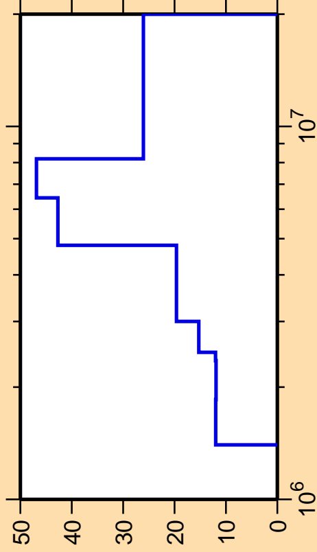
\Delta\sigma/\sigma vs. E for ^{87}\text{Rb}(n,n_4)
