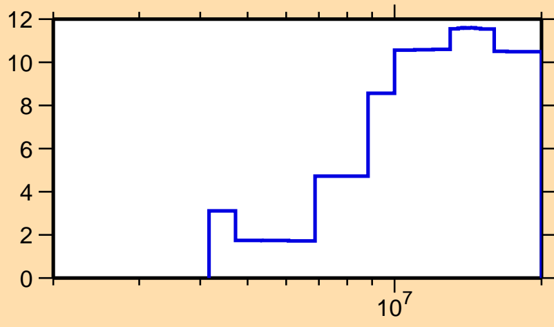
\Delta\sigma/\sigma vs. E for ^{89}\text{Rb}(n,ncont.)
