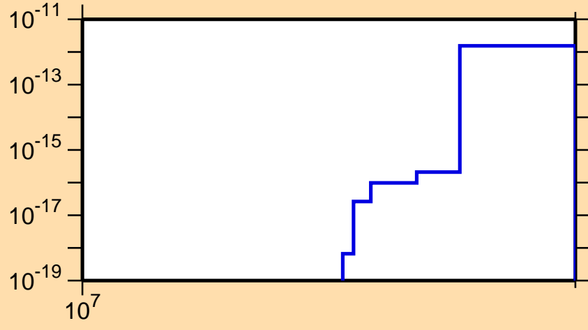
\sigma vs. E for ^{89}\text{Rb}(n,2n\alpha)
