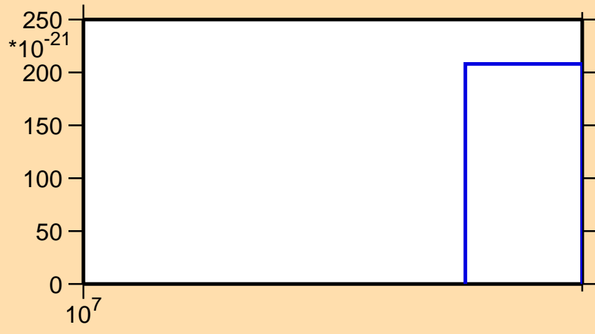
\sigma vs. E for ^{89}\text{Rb} (mt 11)
