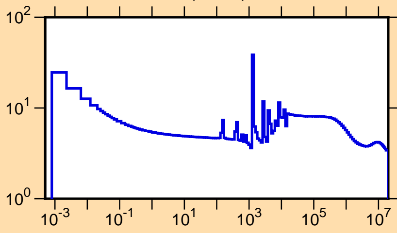
\sigma vs. E for ^{89}\text{Rb}(n,\text{tot.})
