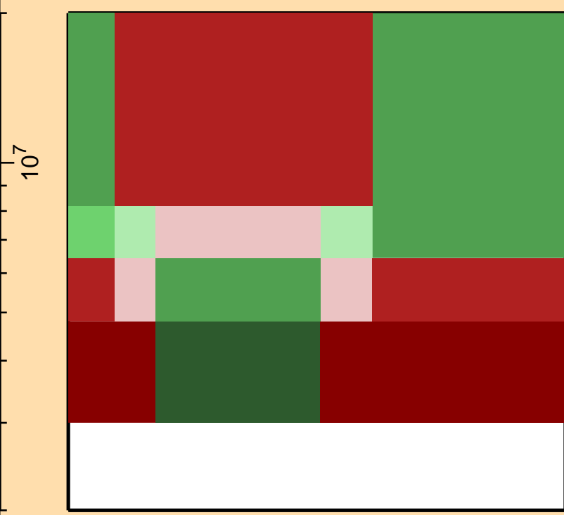
Correlation Matrix
