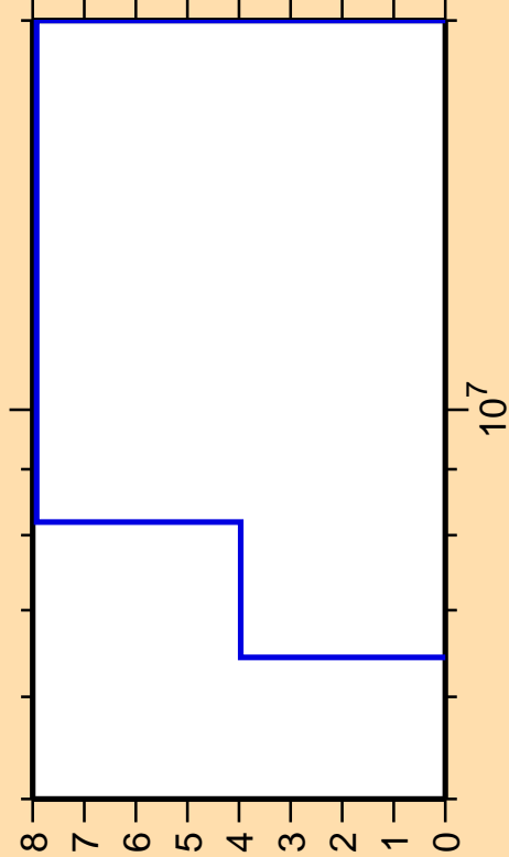
\Delta\sigma/\sigma vs. E for ^{89}\text{Rb}(n,n\text{cont.})
