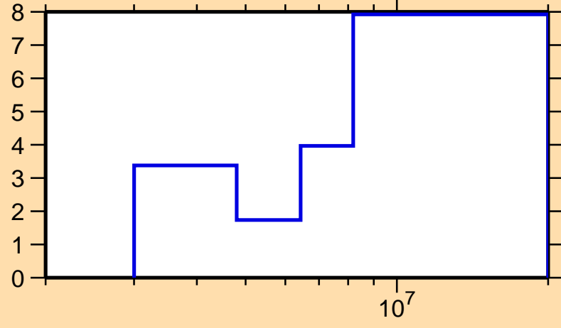
\Delta\sigma/\sigma vs. E for ^{89}\text{Rb}(n,ncont.)
