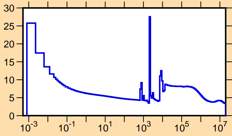
\sigma vs. E for ^{90}\text{Rb}(n,\text{tot.})
