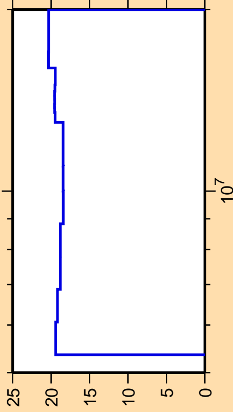
\Delta\sigma/\sigma vs. E for ^{90}\text{Rb}(n,n_1)
