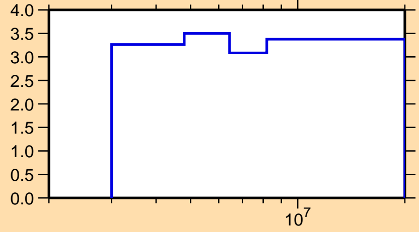
\Delta\sigma/\sigma vs. E for ^{90}\text{Rb}(n,\text{nonel.})
