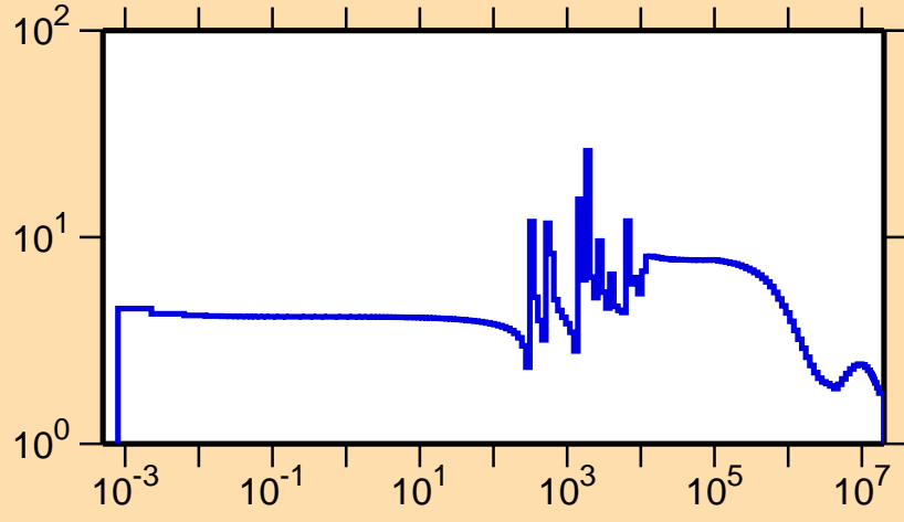
\sigma vs. E for ^{90}\text{Rb}(n,\text{el.})
