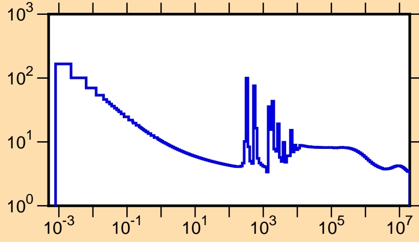
\sigma vs. E for ^{90}\text{Rb}(n,\text{tot.})
