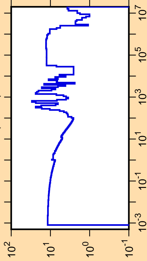
\Delta\sigma/\sigma vs. E for ^{90}\text{Rb}(n,\text{tot.})
