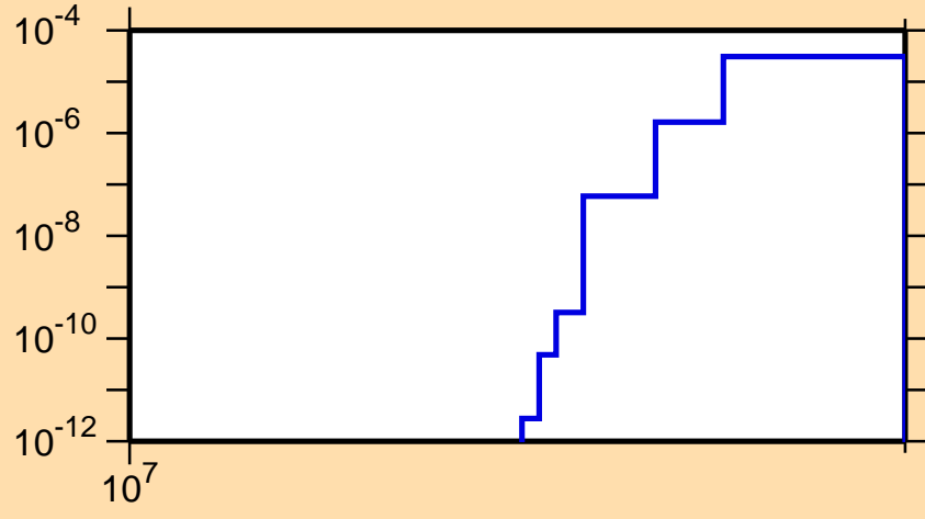
\sigma vs. E for ^{90}\text{Rb}(n,nd)
