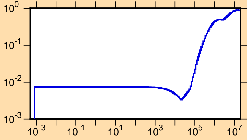
\mu vs. E for ^{91}\text{Rb}(\text{mt251})
