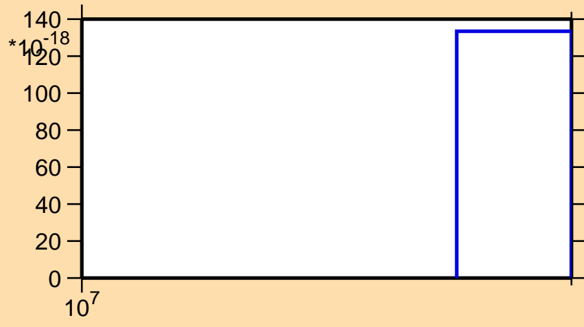
\sigma vs. E for ^{91}\text{Rb} (mt 11)
