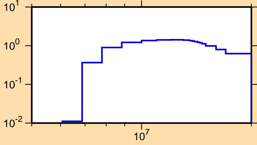
\sigma vs. E for ^{91}\text{Rb}(n,2n)
