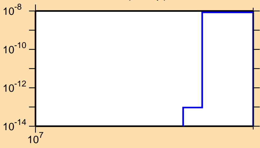
\sigma vs. E for ^{91}\text{Rb}(n,2np)
