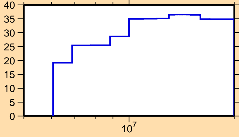
\Delta\sigma/\sigma vs. E for ^{91}\text{Rb}(n,n\text{cont.})
