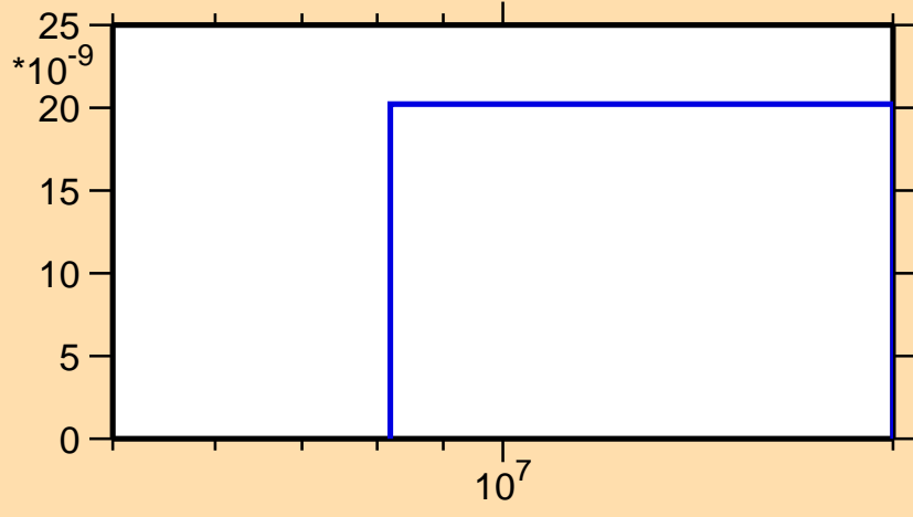
\sigma vs. E for ^{91}\text{Rb}(n,\text{nd})
