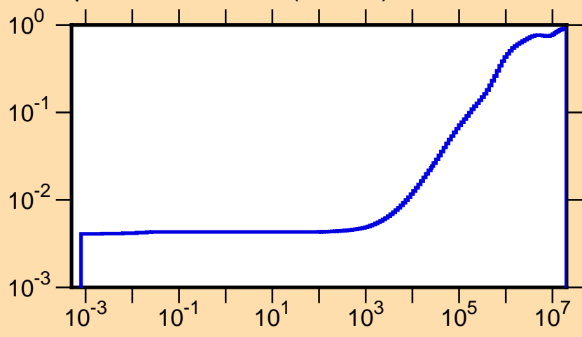
\mu vs. E for ^{165}\text{Re}(\text{mt251})
