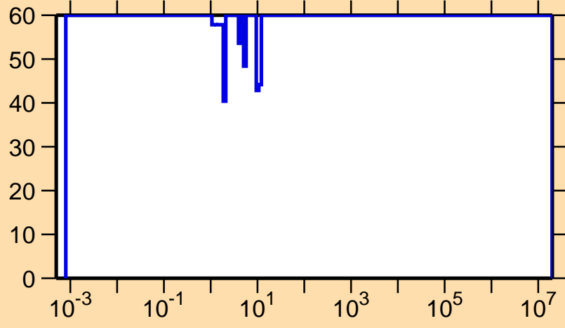
\Delta\sigma/\sigma vs. E for ^{165}\text{Re}(n,\gamma)
