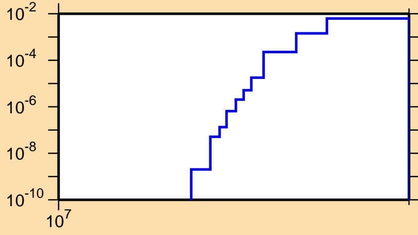
\sigma vs. E for ^{165}\text{Re}(n,2np)
