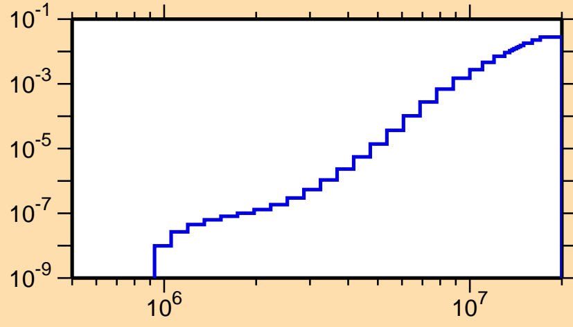
\sigma vs. E for ^{165}\text{Re}(n,n\alpha)
