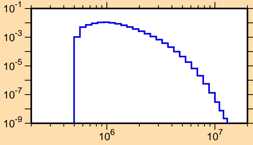
\sigma vs. E for ^{165}\text{Re}(n,n_2)
