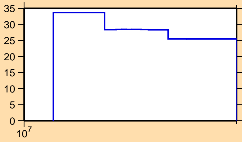
\Delta\sigma/\sigma vs. E for ^{165}\text{Re}(n,\text{nonel.})
