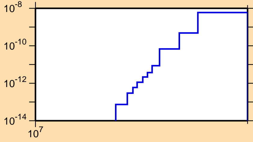
\sigma vs. E for ^{165}\text{Re}(\text{mt } 34)
