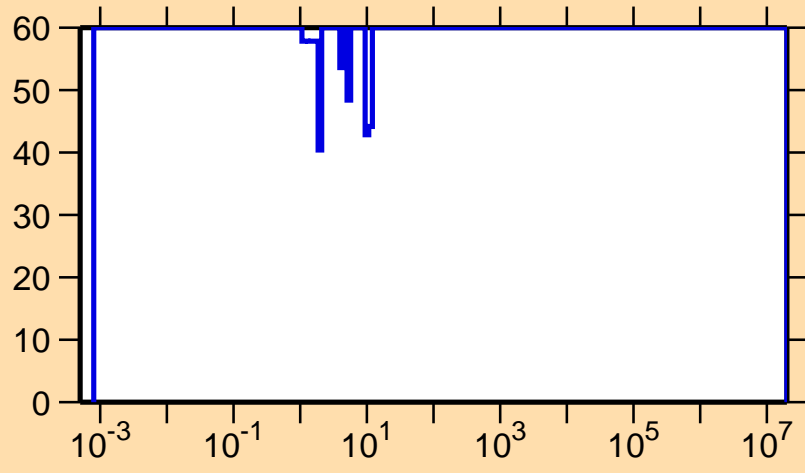
\Delta\sigma/\sigma vs. E for ^{165}\text{Re}(n,\gamma)
