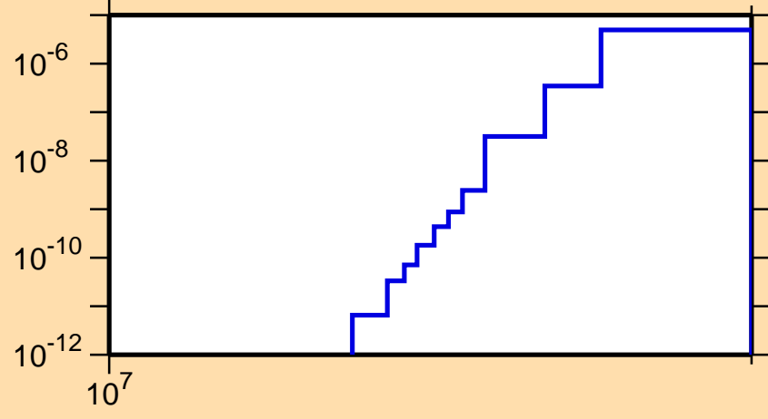
\sigma vs. E for ^{165}\text{Re}(n,\text{pt})
