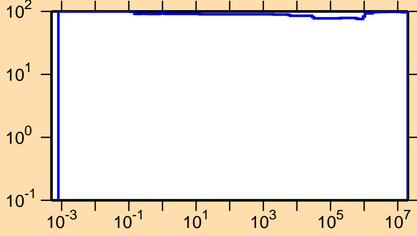
\Delta\sigma/\sigma vs. E for ^{165}\text{Re}(n,p)
