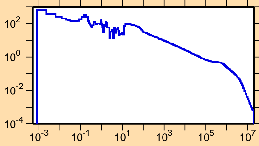
\sigma vs. E for ^{165}\text{Re}(n,\gamma)
