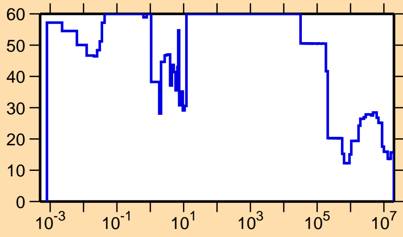
\Delta\sigma/\sigma vs. E for ^{165}\text{Re}(n,\text{tot.})
