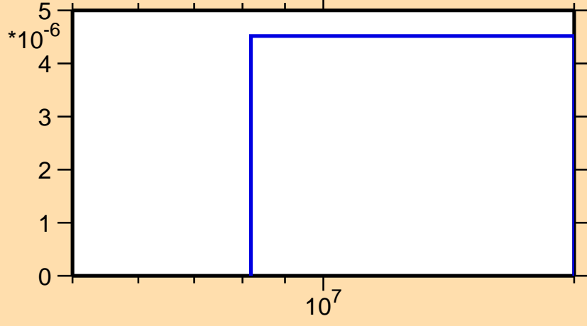
\sigma vs. E for ^{166}\text{Re}(n,\text{nd})
