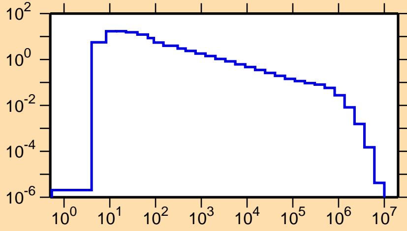
\sigma vs. E for ^{167}\text{Re}(n,n_1)
