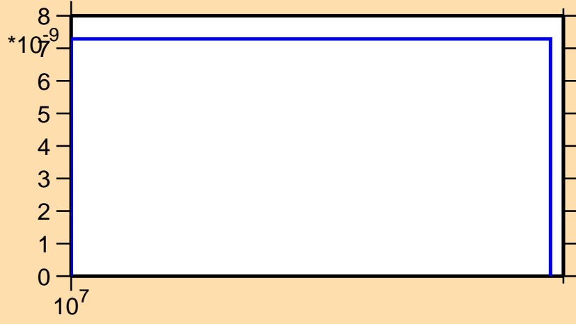
\sigma vs. E for ^{167}\text{Re}(n,\text{pt})
