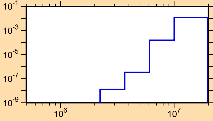
\sigma vs. E for ^{167}\text{Re}(n,d)
