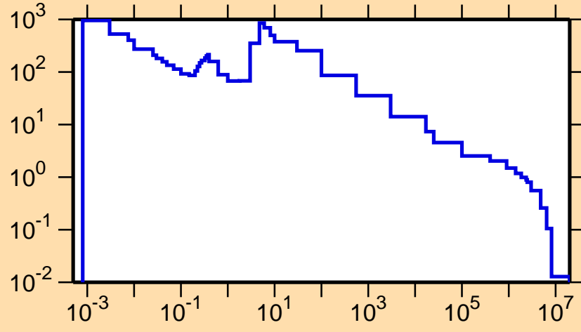
\sigma vs. E for ^{167}\text{Re}(n,\gamma)
