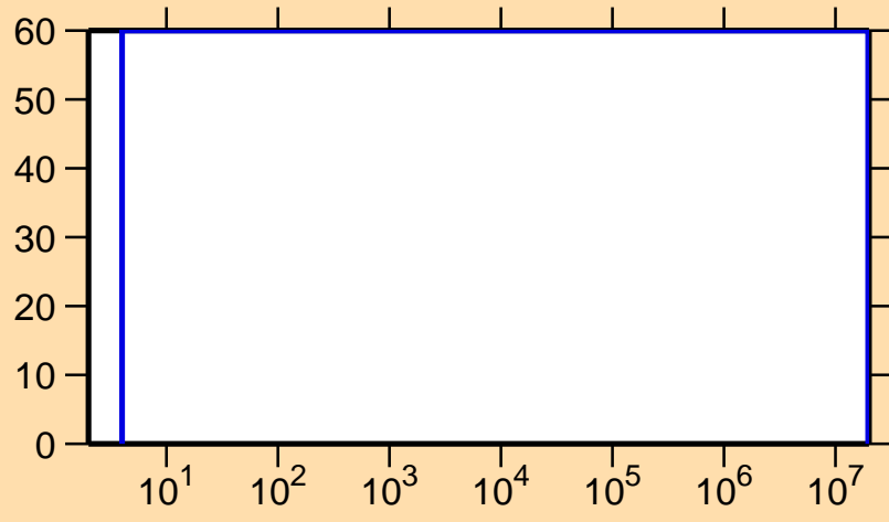
\Delta\sigma/\sigma vs. E for ^{169}\text{Re}(n,n_1)
