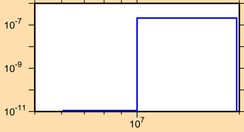
\sigma vs. E for ^{169}\text{Re}(\text{mt117})
