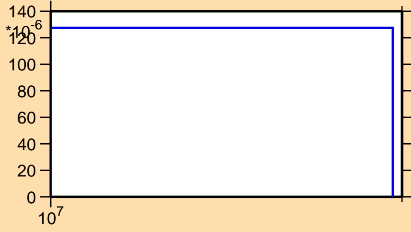
\sigma vs. E for ^{169}\text{Re}(n,2np)
