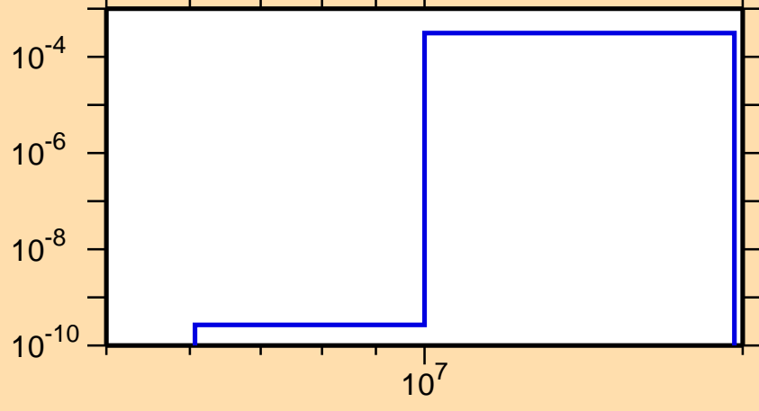
\sigma vs. E for ^{169}\text{Re}(n,t)
