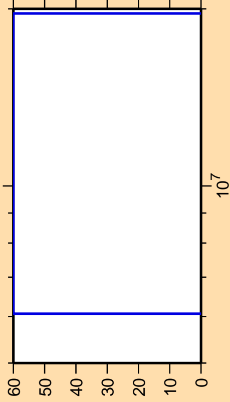
\Delta\sigma/\sigma vs. E for ^{169}\text{Re}(n,t)
