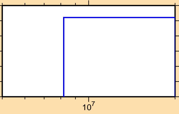
\sigma vs. E for ^{169}\text{Re}(n,2np)
