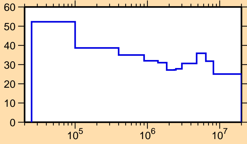
\Delta\sigma/\sigma vs. E for ^{169}\text{Re}(n,n\text{onel.})
