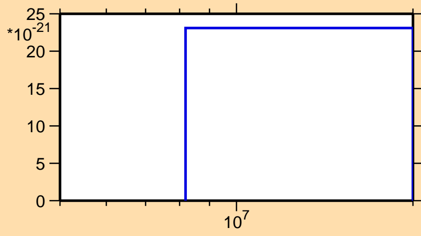
\sigma vs. E for ^{169}\text{Re}(\text{mt } 42)
