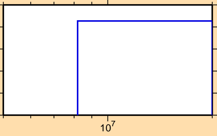
\sigma vs. E for ^{169}\text{Re}(n,\text{pd})
