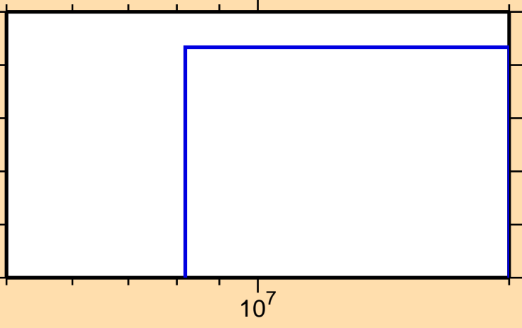
\sigma vs. E for ^{169}\text{Re}(n,3n)
