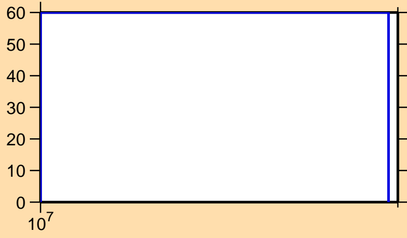
\Delta\sigma/\sigma vs. E for ^{171}\text{Re}(n,2n)
