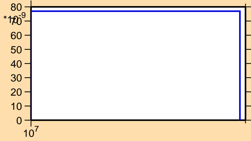
\sigma vs. E for ^{171}\text{Re}(n,\text{nd})
