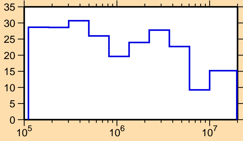
\Delta\sigma/\sigma vs. E for ^{171}\text{Re}(n,\text{tot.})
