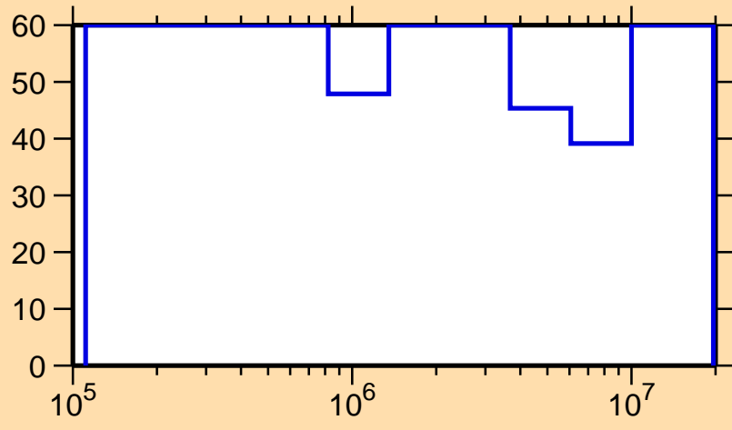
\Delta\sigma/\sigma vs. E for ^{171}\text{Re}(n,\text{inel.})
