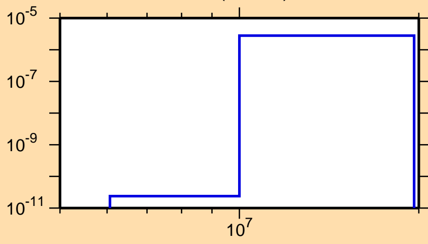
\sigma vs. E for ^{171}\text{Re}(n,\text{He3})
