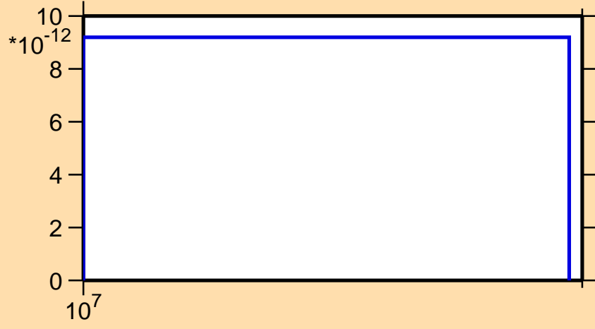
\sigma vs. E for ^{171}\text{Re}(n,\text{pt})
