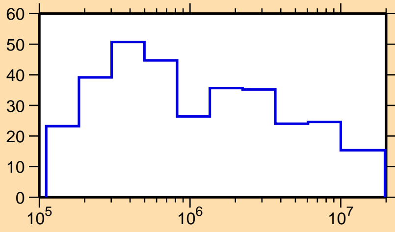
\Delta\sigma/\sigma vs. E for ^{171}\text{Re}(n,\text{el.})
