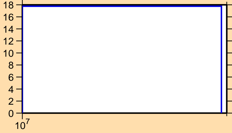
\Delta\sigma/\sigma vs. E for ^{171}\text{Re}(n,\text{nonel.})
