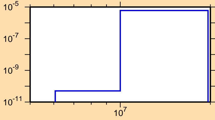
\sigma vs. E for ^{171}\text{Re}(\text{mt } 45)
