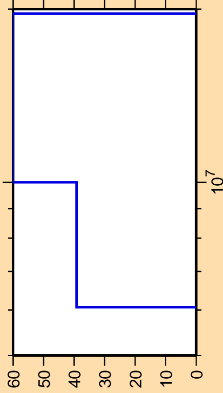
\Delta\sigma/\sigma vs. E for ^{171}\text{Re}(\text{mt } 45)
