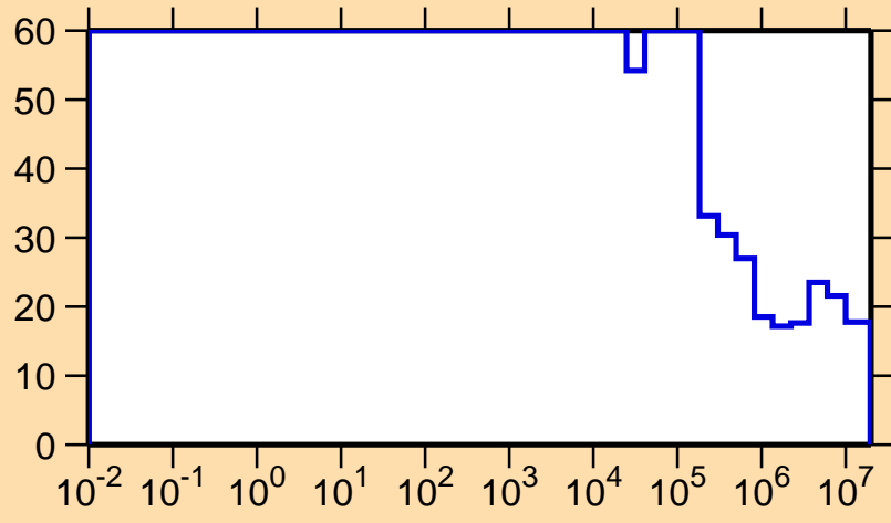
\Delta\sigma/\sigma vs. E for ^{171}\text{Re}(n,\text{nonel.})
