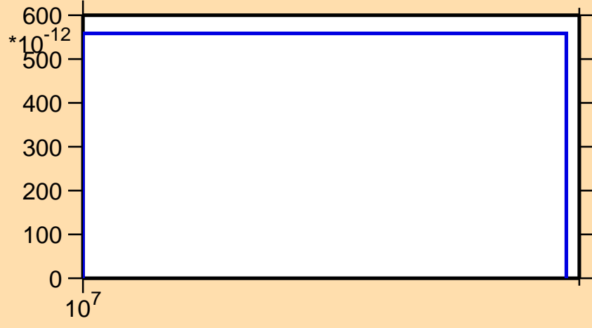
\sigma vs. E for ^{171}\text{Re}(n,nt)
