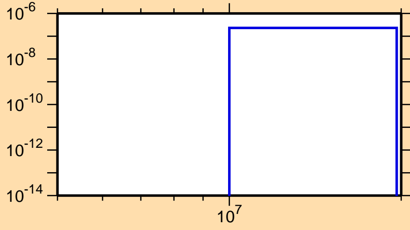
\sigma vs. E for ^{171}\text{Re}(n,2n\alpha)
