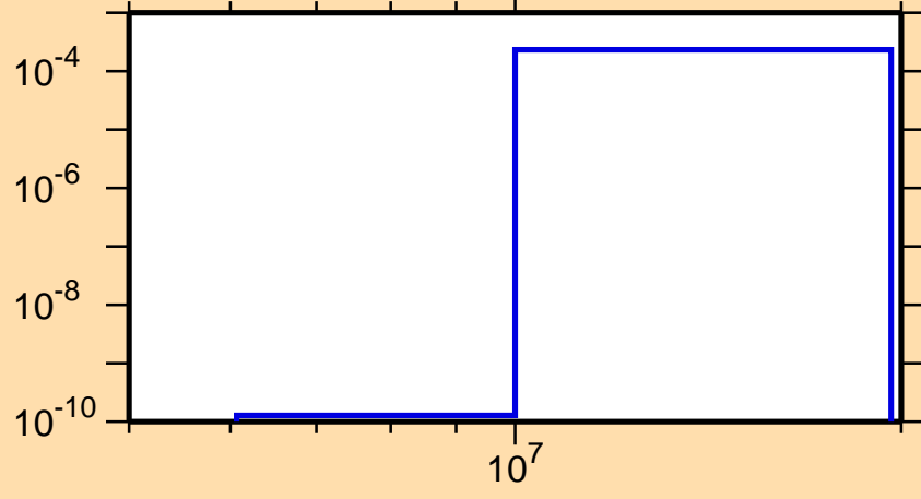
\sigma vs. E for ^{171}\text{Re}(n,t)
