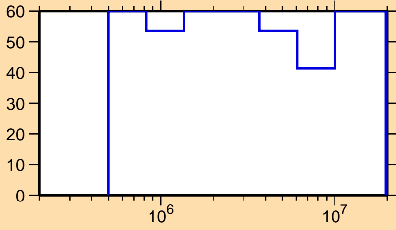
\Delta\sigma/\sigma vs. E for ^{171}\text{Re}(n,n\text{cont.})
