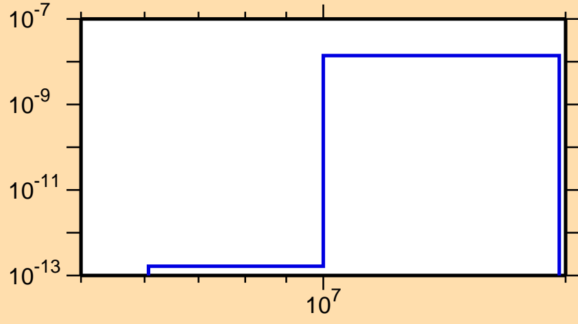
\sigma vs. E for ^{171}\text{Re}(\text{mt117})
