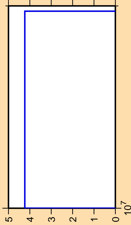
\Delta\sigma/\sigma vs. E for ^{171}\text{Re}(\text{mt } 34)
