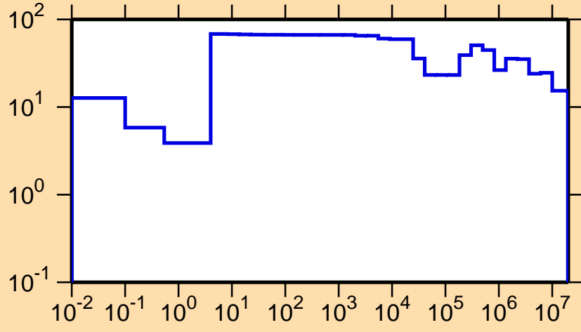
\Delta\sigma/\sigma vs. E for ^{171}\text{Re}(n,\text{el.})
