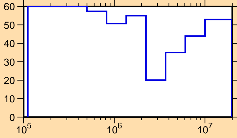
\Delta\sigma/\sigma vs. E for ^{171}\text{Re}(n,n_1)
