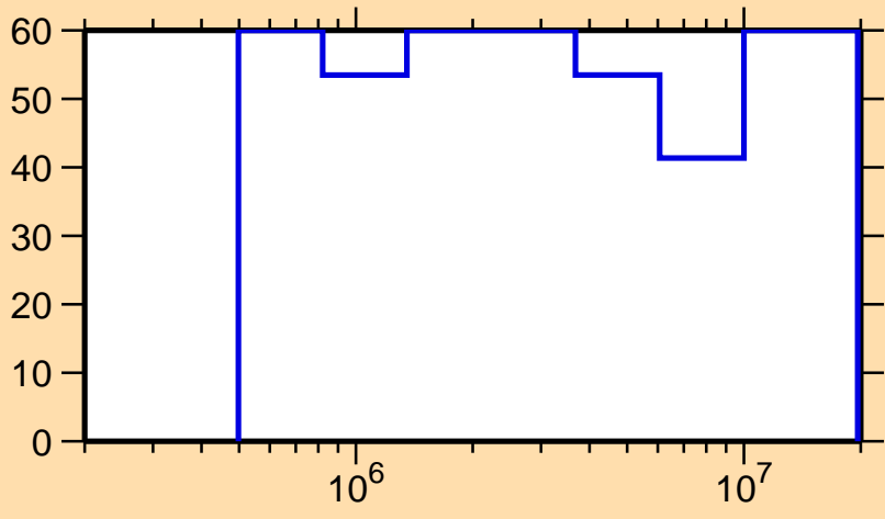
\Delta\sigma/\sigma vs. E for ^{171}\text{Re}(n,n\text{cont.})
