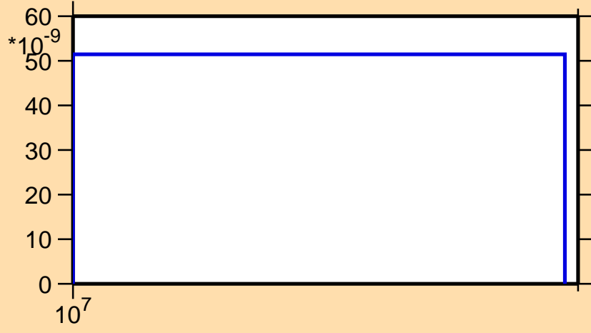
\sigma vs. E for ^{171}\text{Re}(n,3n)
