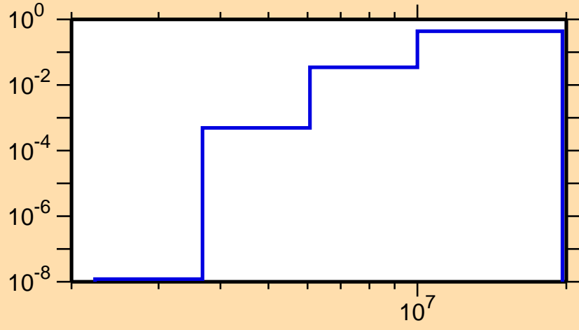
\sigma vs. E for ^{171}\text{Re}(n,np)
