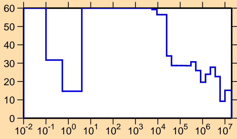
\Delta\sigma/\sigma vs. E for ^{171}\text{Re}(n,\text{tot.})
