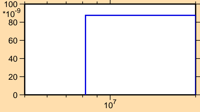
\sigma vs. E for ^{171}\text{Re}(n,3n)
