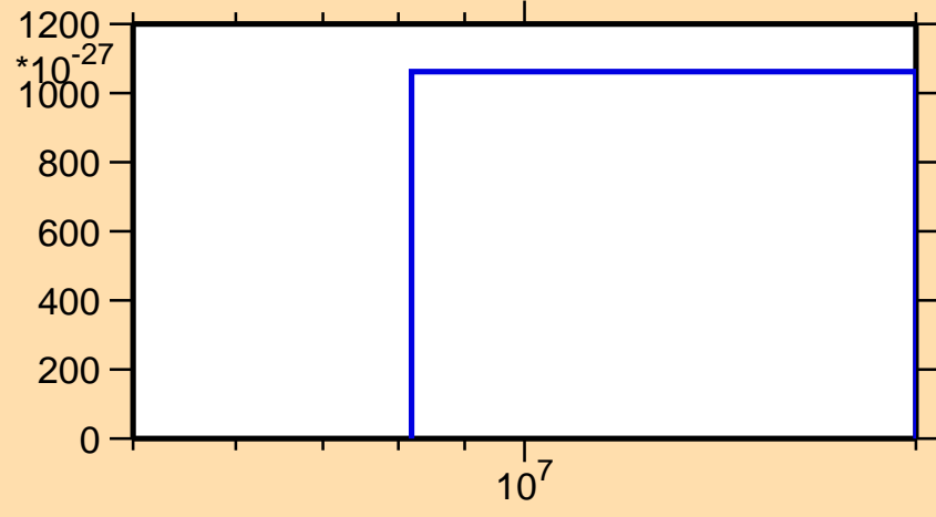
\sigma vs. E for ^{171}\text{Re}(\text{mt } 42)
