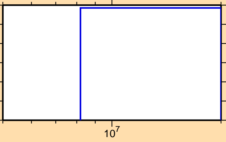
\sigma vs. E for ^{171}\text{Re}(n,2np)
