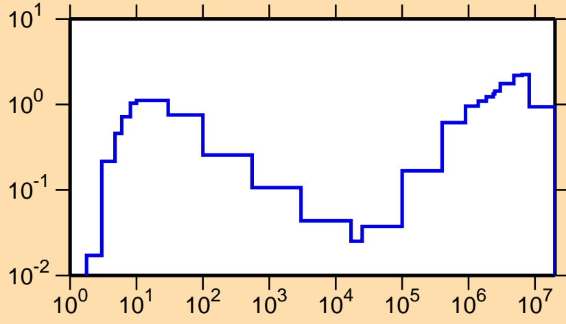
\sigma vs. E for ^{172}\text{Re}(n,\text{inel.})
