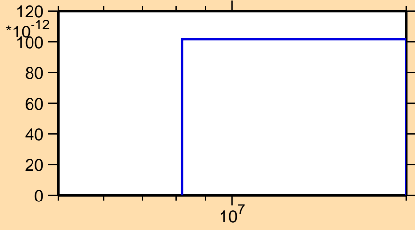
\sigma vs. E for ^{172}\text{Re}(\text{mt } 34)
