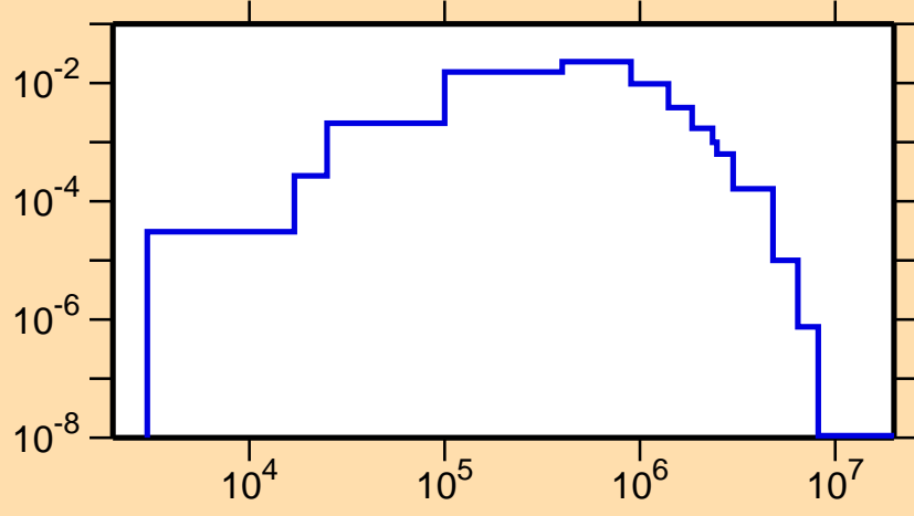
\sigma vs. E for ^{172}\text{Re}(n,n_2)
