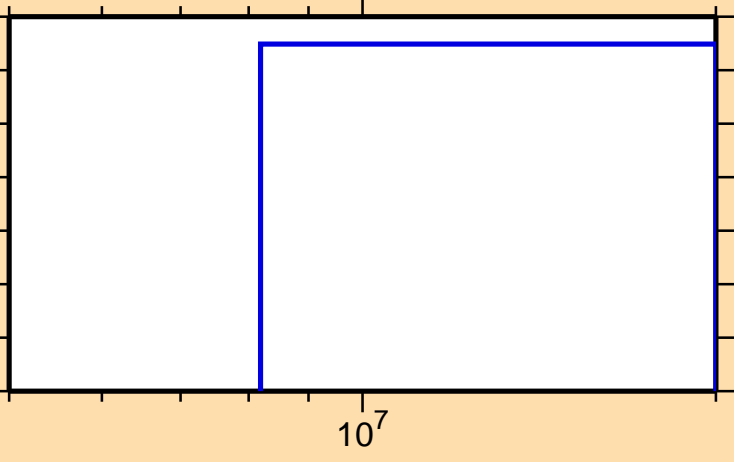
\sigma vs. E for ^{172}\text{Re}(n,3n)
