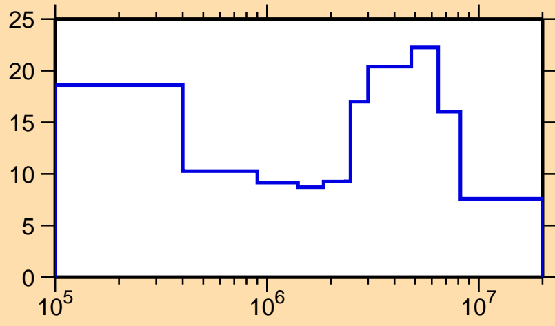
\Delta\sigma/\sigma vs. E for ^{172}\text{Re}(n, el.)
