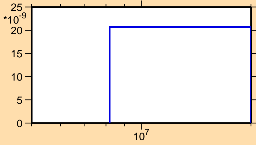
\sigma vs. E for ^{172}\text{Re}(n,\text{pd})
