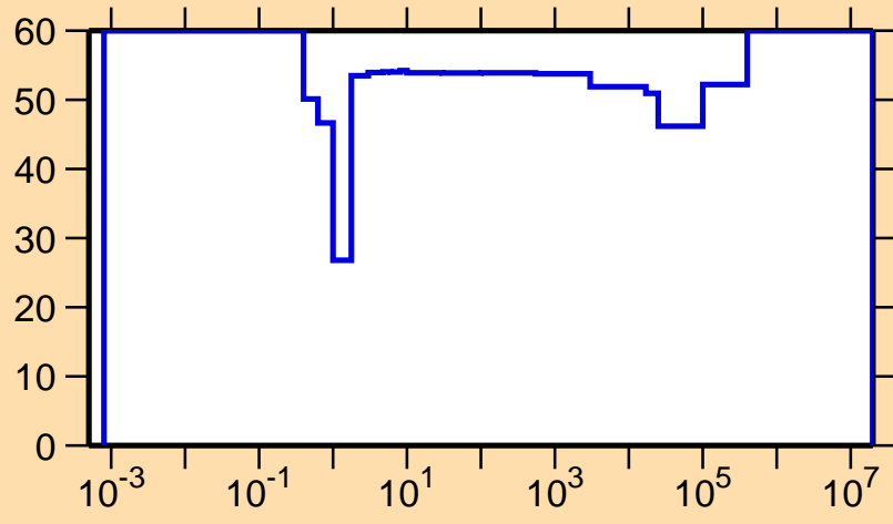
\Delta\sigma/\sigma vs. E for ^{172}\text{Re}(n,\gamma)
