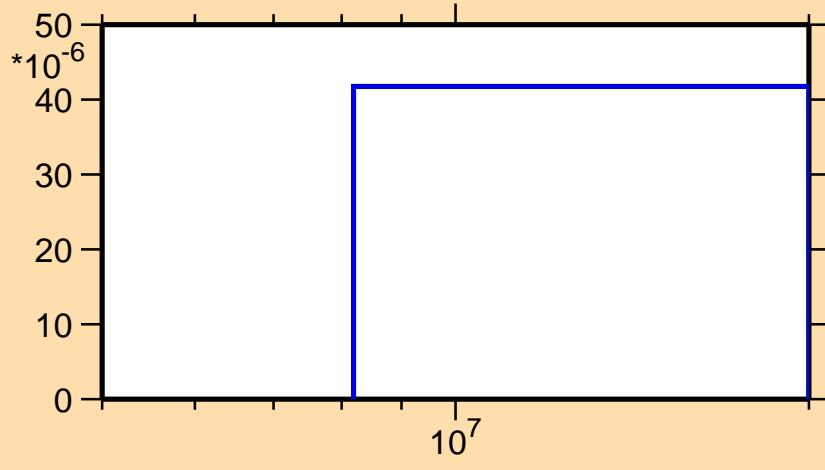
\sigma vs. E for ^{172}\text{Re}(n,2n\alpha)
