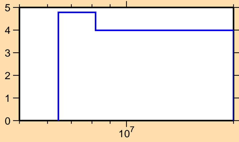
\Delta\sigma/\sigma vs. E for ^{172}\text{Re}(n,\text{nonel.})
