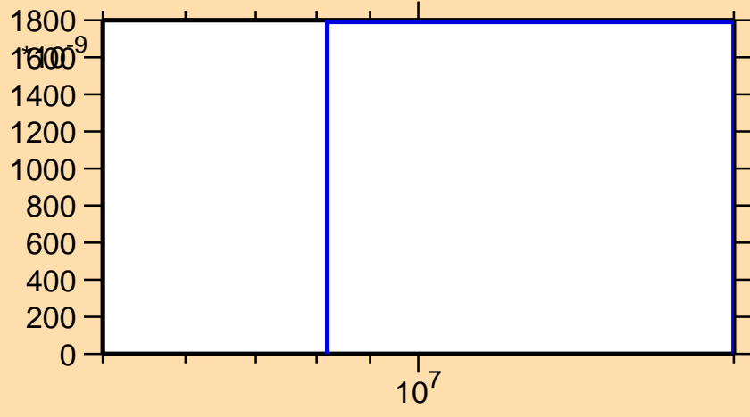
\sigma vs. E for ^{172}\text{Re}(\text{mt } 45)
