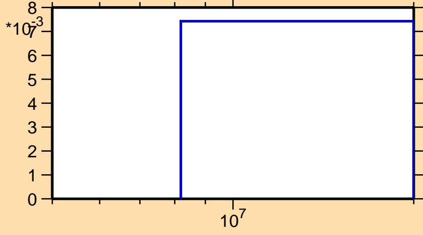
\sigma vs. E for ^{172}\text{Re}(n,2np)
