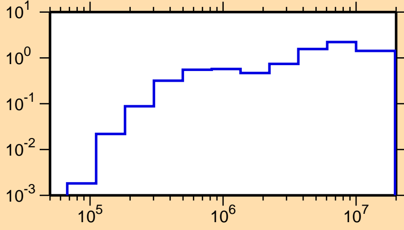
\sigma vs. E for ^{173}\text{Re}(n,\text{inel.})
