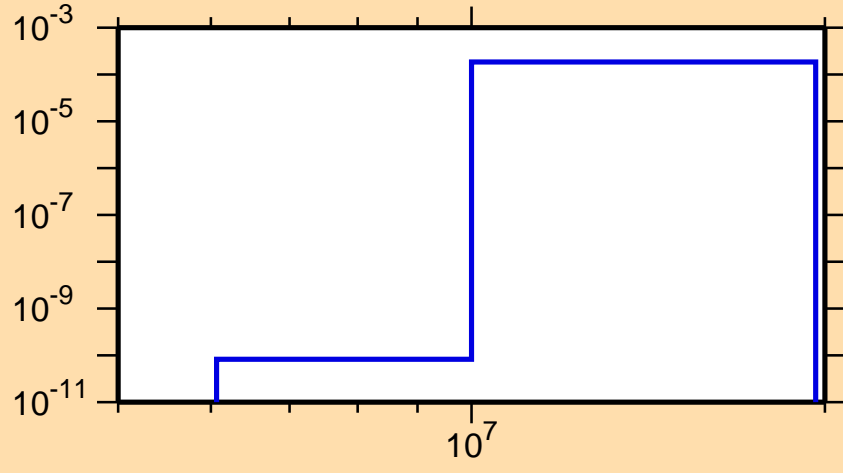
\sigma vs. E for ^{173}\text{Re}(n,t)
