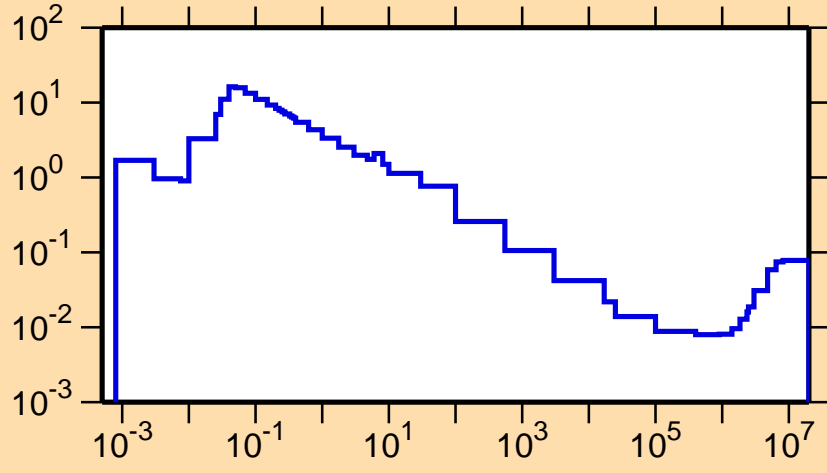
\sigma vs. E for ^{173}\text{Re}(n,p)
