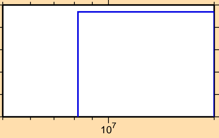
\sigma vs. E for ^{173}\text{Re}(n,\text{nd})
