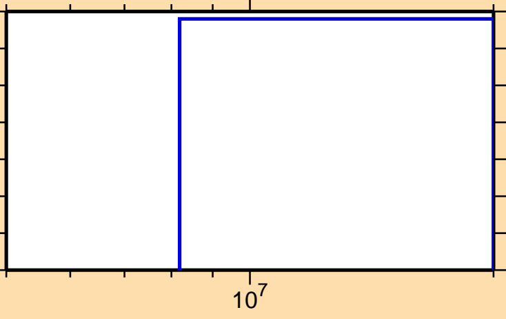
\sigma vs. E for ^{173}\text{Re}(\text{mt } 34)
