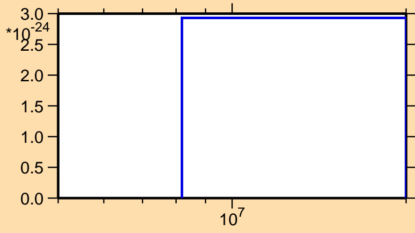
\sigma vs. E for ^{173}\text{Re}(\text{mt } 42)
