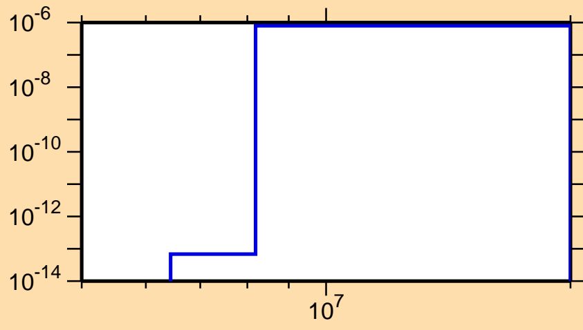
\sigma vs. E for ^{173}\text{Re}(n,\text{He3})
