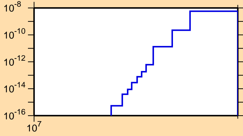
\sigma vs. E for ^{174}\text{Re}(n,\text{pt})
