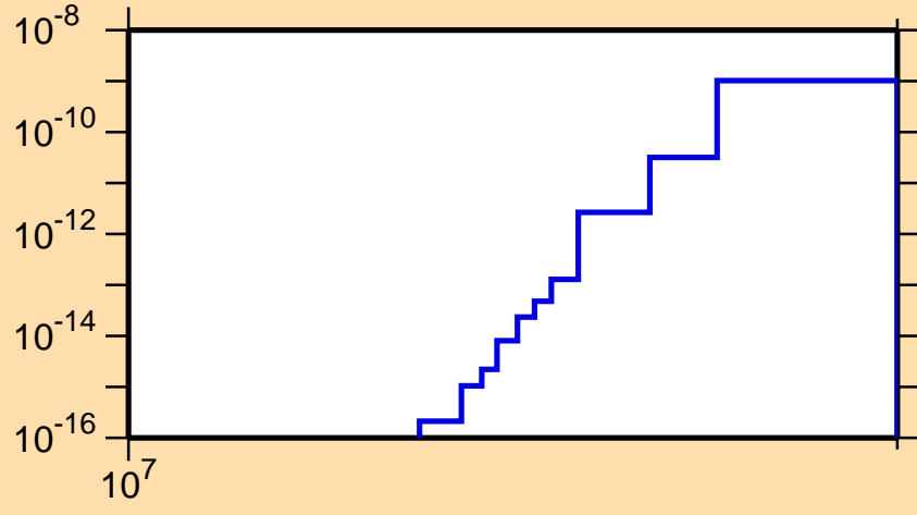
\sigma vs. E for ^{174}\text{Re}(\text{mt } 34)
