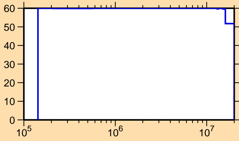
\Delta\sigma/\sigma vs. E for ^{174}\text{Re}(n,n_1)
