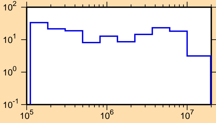
\Delta\sigma/\sigma vs. E for ^{174}\text{Re}(n, el.)
