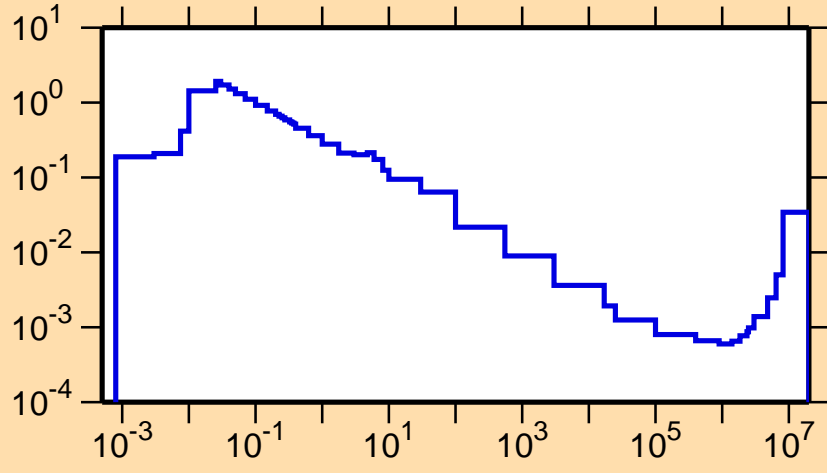
\sigma vs. E for ^{174}\text{Re}(n,\alpha)
