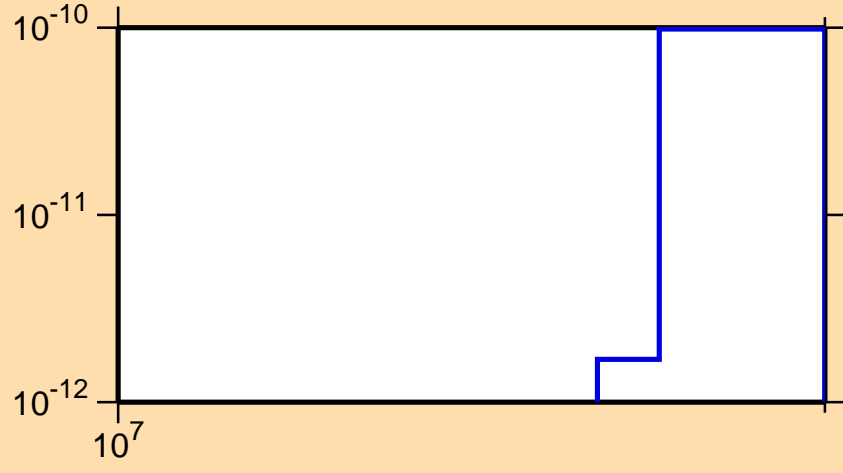
\sigma vs. E for ^{176}\text{Re}(\text{mt 34})
