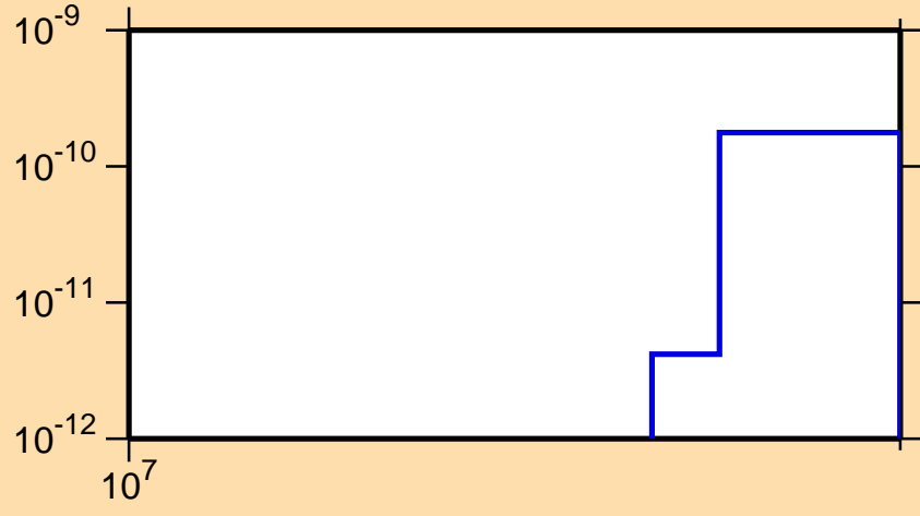
\sigma vs. E for ^{176}\text{Re}(n,\text{pt})
