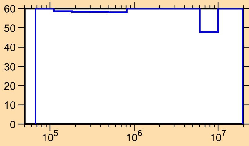
\Delta\sigma/\sigma vs. E for ^{176}\text{Re}(n,n_1)
