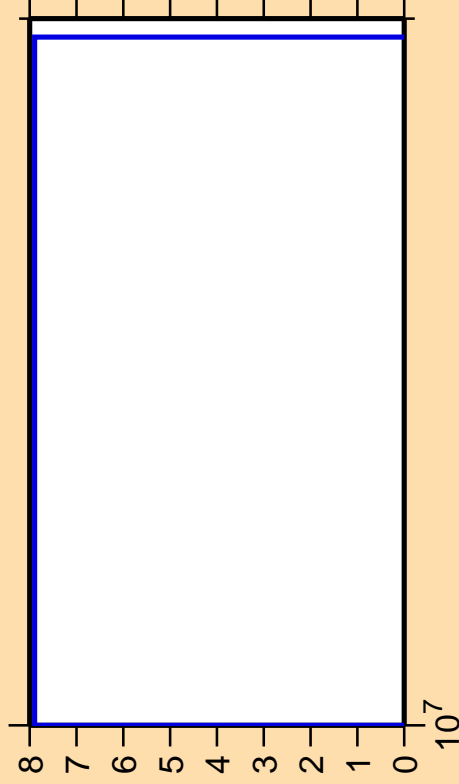
\Delta\sigma/\sigma vs. E for ^{176}\text{Re}(n,\text{pt})
