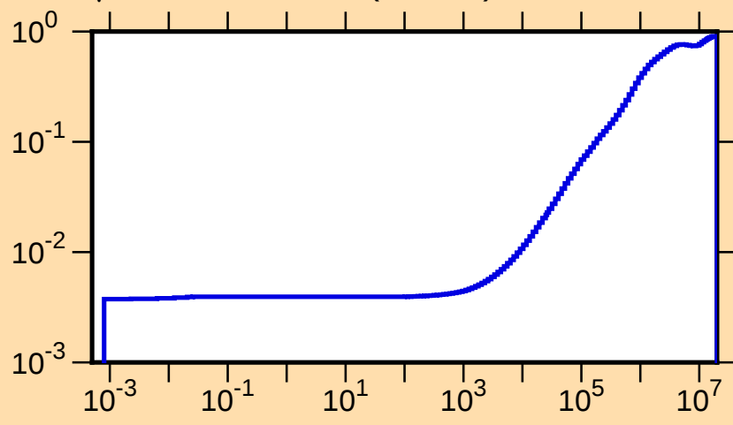
\mu vs. E for ^{180}\text{Re}(\text{mt251})
