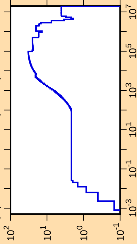
\Delta\mu/\mu vs. E for ^{180}\text{Re}(\text{mt251})
