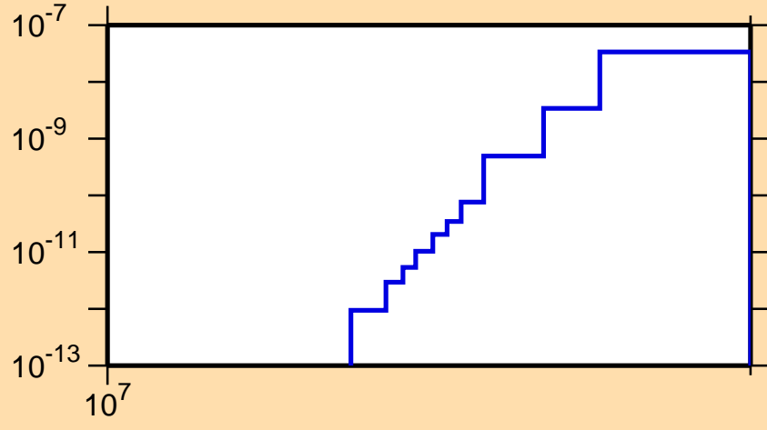
\sigma vs. E for ^{181}\text{Re}(n,\text{He3})
