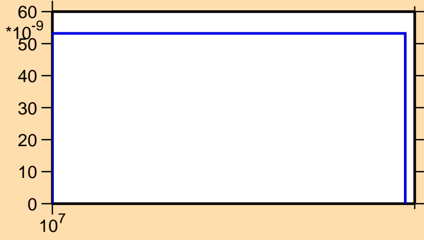
\sigma vs. E for ^{181}\text{Re}(n,nd)
