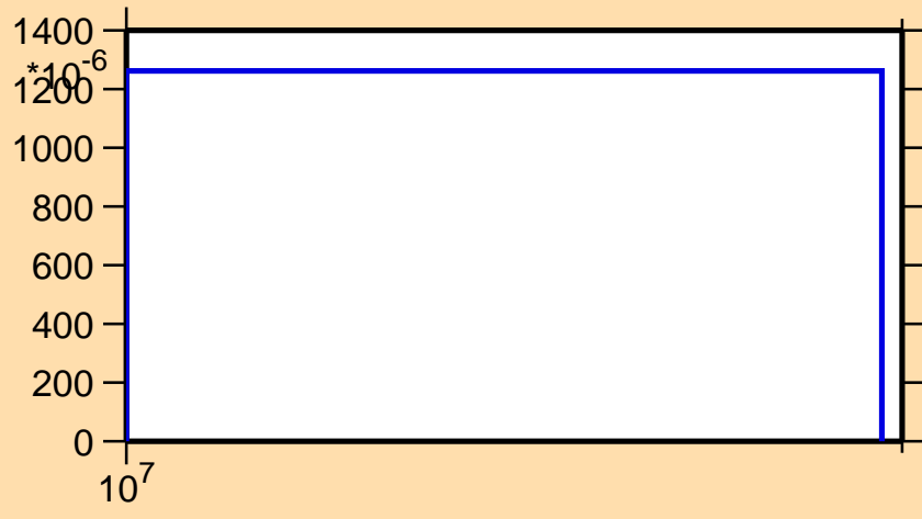
\sigma vs. E for ^{181}\text{Re}(n,3n)
