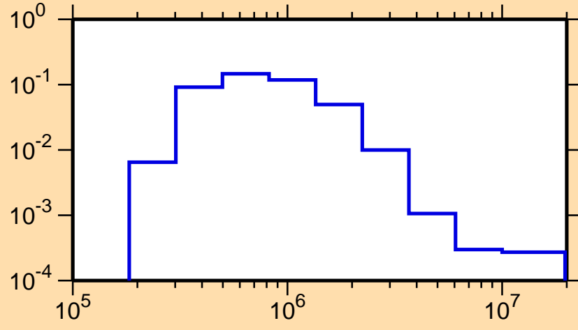
\sigma vs. E for ^{181}\text{Re}(n,n_3)
