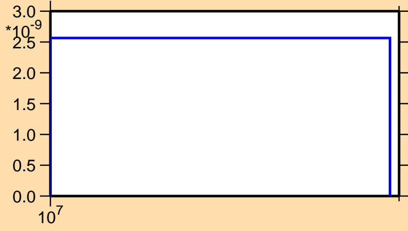
\sigma vs. E for ^{181}\text{Re}(n,nt)
