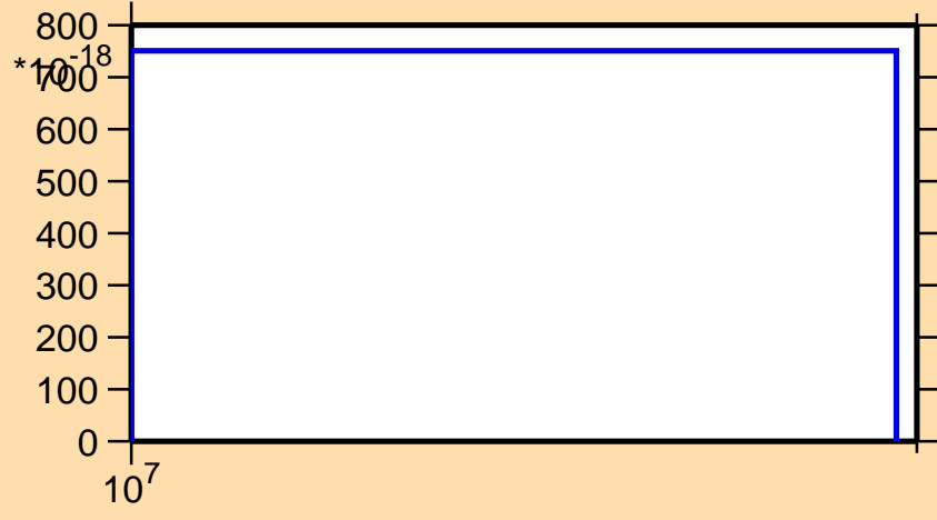
\sigma vs. E for ^{181}\text{Re}(n,pd)
