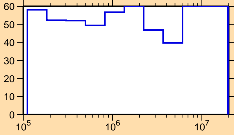
\Delta\sigma/\sigma vs. E for ^{181}\text{Re}(n,n_1)
