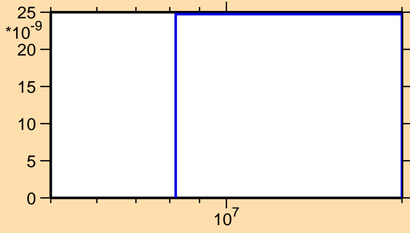
\sigma vs. E for ^{181}\text{Re}(n,2n\alpha)
