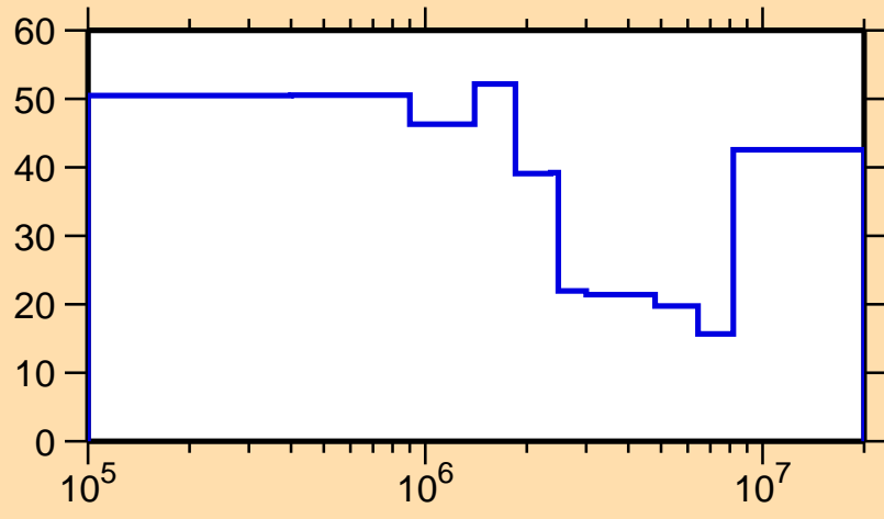
\Delta\sigma/\sigma vs. E for ^{181}\text{Re}(n,\text{inel.})
