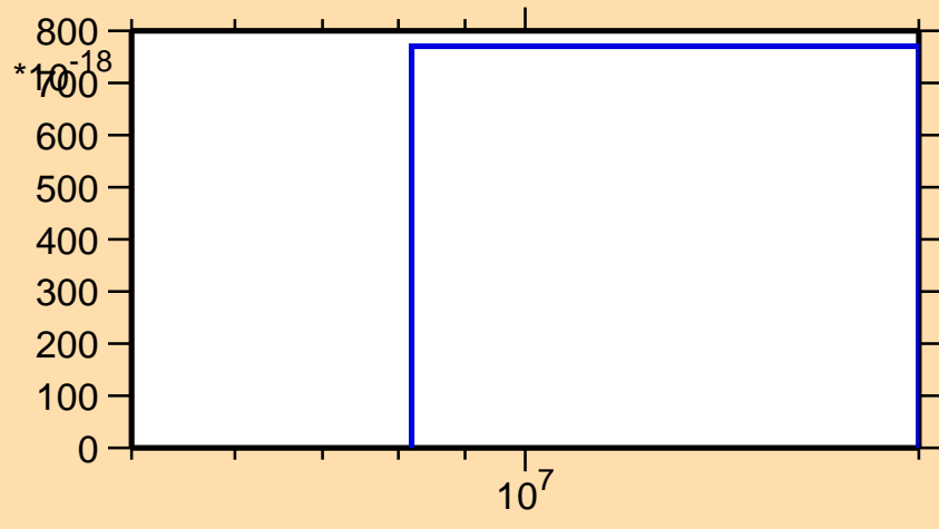
\sigma vs. E for ^{181}\text{Re}(n,pd)
