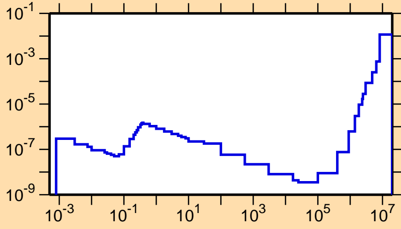
\sigma vs. E for ^{181}\text{Re}(n,p)
