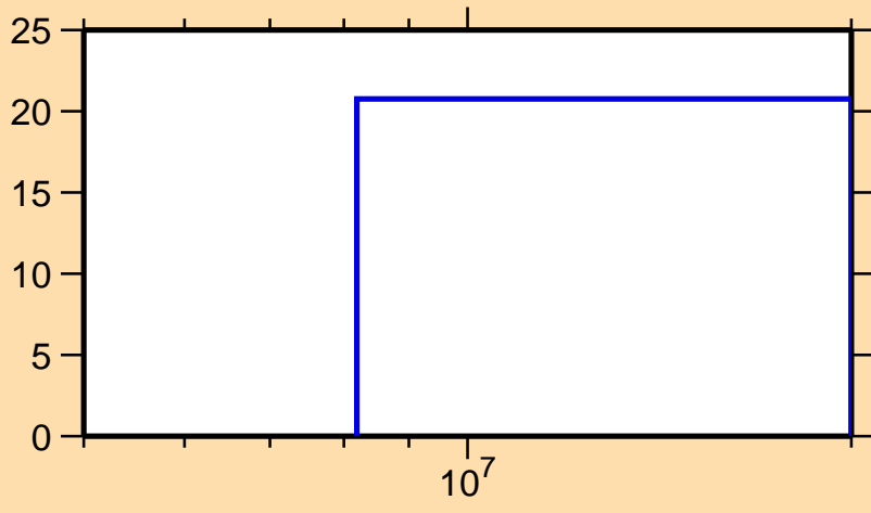
\Delta\sigma/\sigma vs. E for ^{181}\text{Re}(n,2n)
