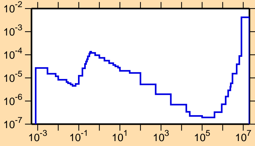
\sigma vs. E for ^{181}\text{Re}(n,\alpha)
