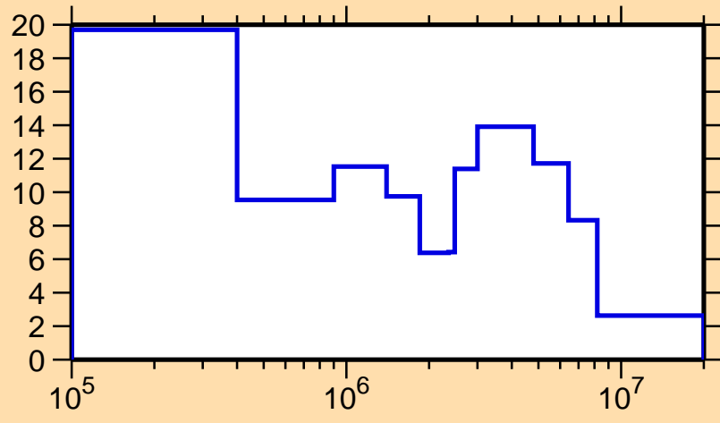
\Delta\sigma/\sigma vs. E for ^{181}\text{Re}(n,\text{tot.})
