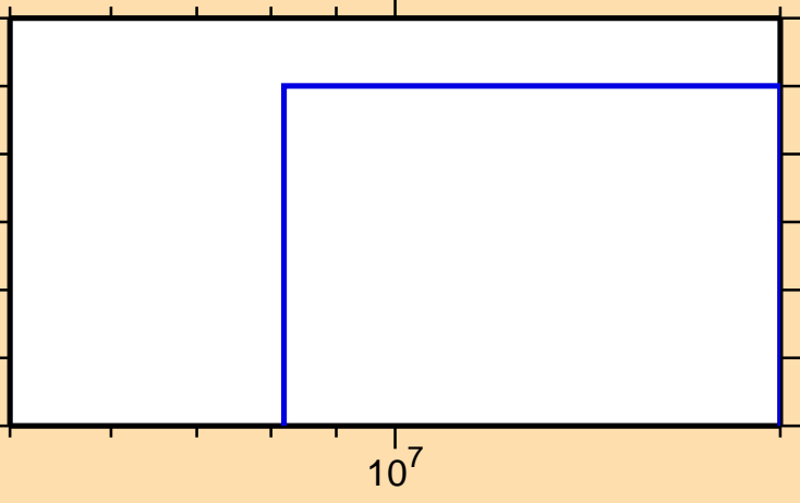
\sigma vs. E for ^{181}\text{Re}(n,nt)
