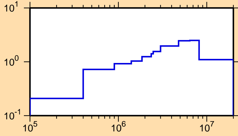
\sigma vs. E for ^{181}\text{Re}(n,\text{inel.})
