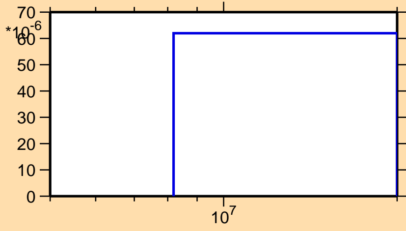
\sigma vs. E for ^{181}\text{Re}(n,t)
