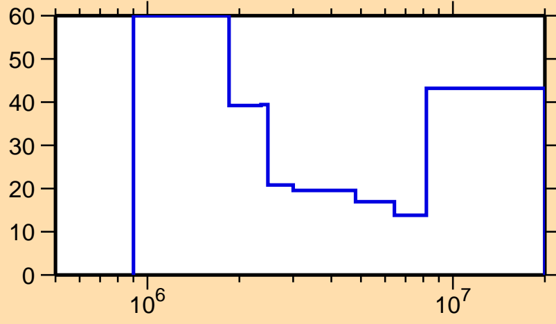
\Delta\sigma/\sigma vs. E for ^{181}\text{Re}(n,n\text{cont.})
