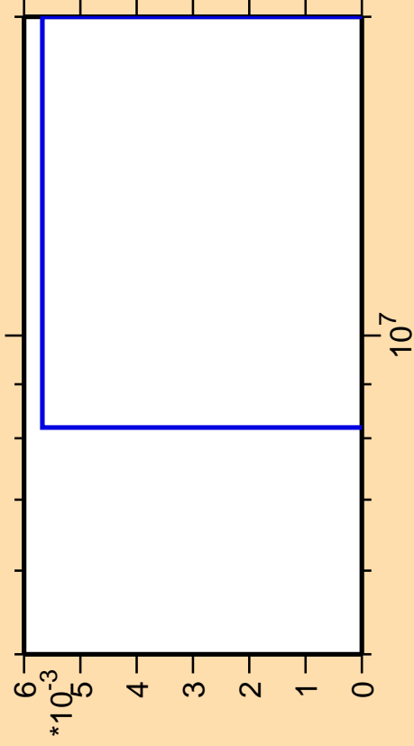
\Delta\sigma/\sigma vs. E for ^{181}\text{Re}(n,pd)
