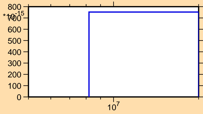
\sigma vs. E for ^{181}\text{Re}(\text{mt } 45)
