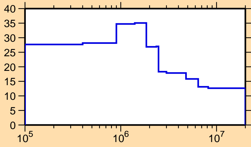
\Delta\sigma/\sigma vs. E for ^{181}\text{Re}(n,\text{nonel.})
