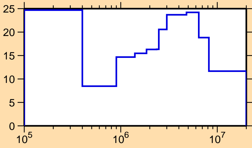
\Delta\sigma/\sigma vs. E for ^{181}\text{Re}(n,\text{el.})
