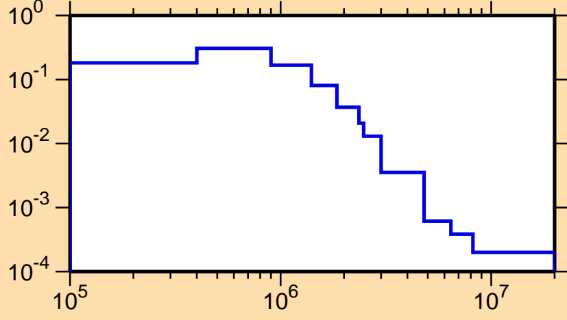
\sigma vs. E for ^{181}\text{Re}(n,n_1)
