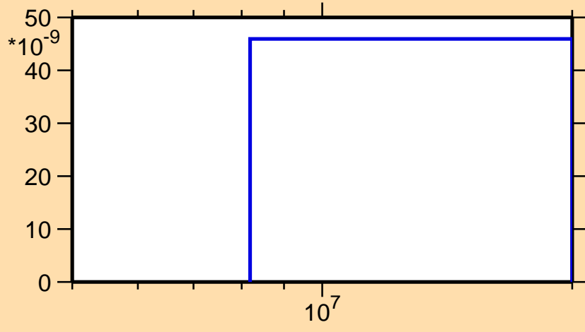
\sigma vs. E for ^{181}\text{Re}(n,\text{nd})
