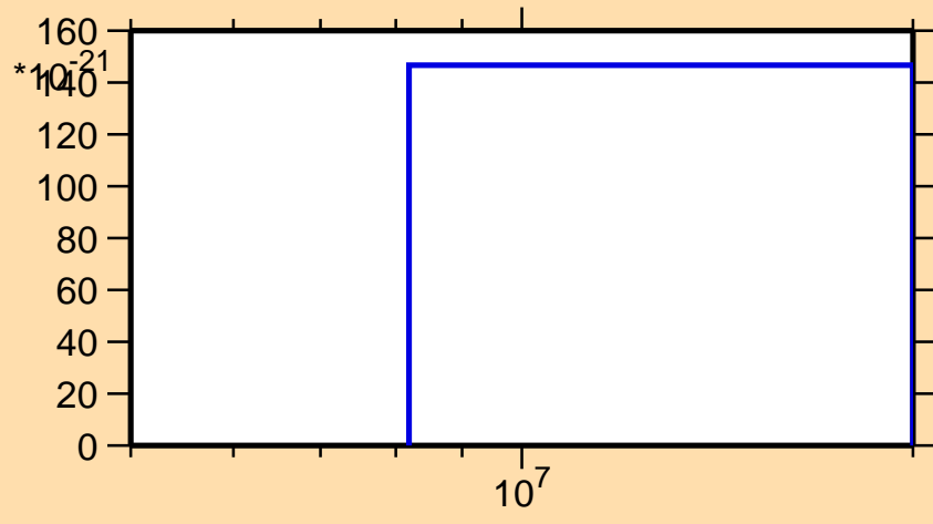
\sigma vs. E for ^{181}\text{Re}(\text{mt } 42)
