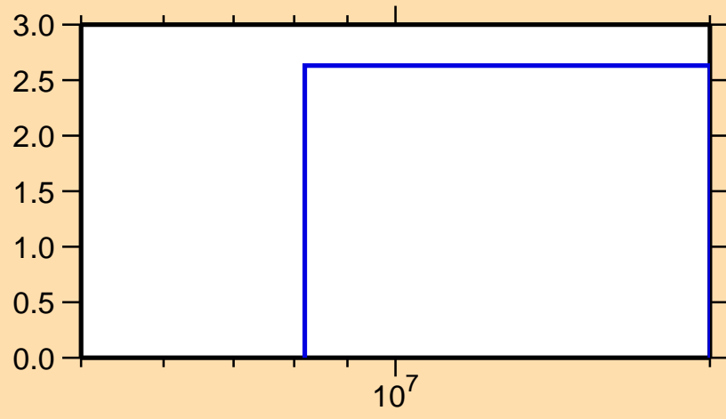
\Delta\sigma/\sigma vs. E for ^{181}\text{Re}(n,\text{tot.})
