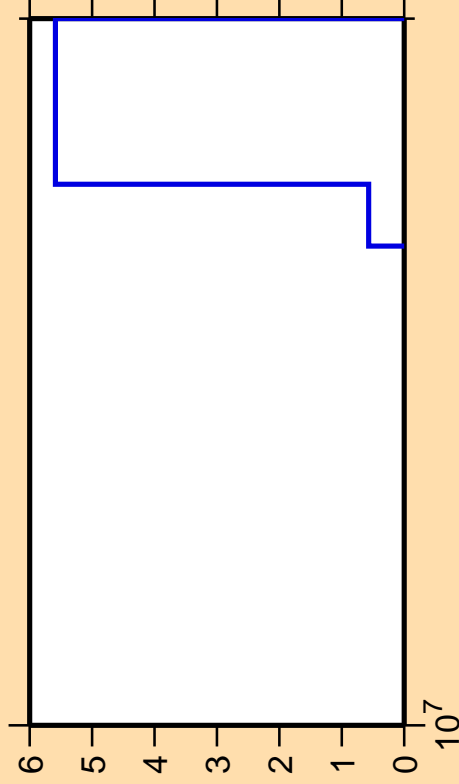
\Delta\sigma/\sigma vs. E for ^{182}\text{Re}(\text{mt } 45)
