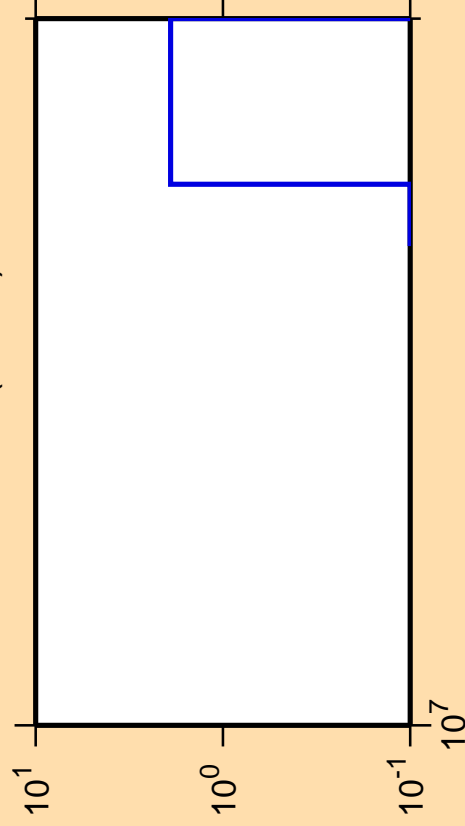
\Delta\sigma/\sigma vs. E for ^{182}\text{Re}(\text{mt } 34)
