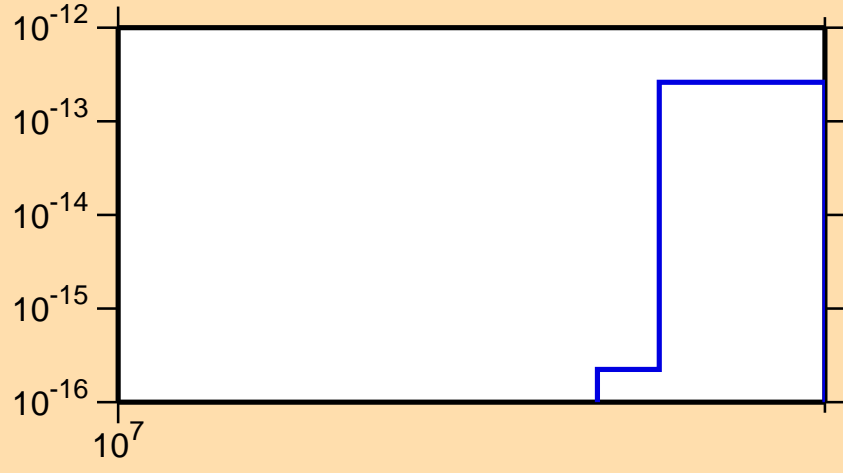
\sigma vs. E for ^{182}\text{Re}(\text{mt } 34)
