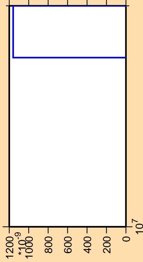
\Delta\sigma/\sigma vs. E for ^{182}\text{Re}(\text{mt } 42)
