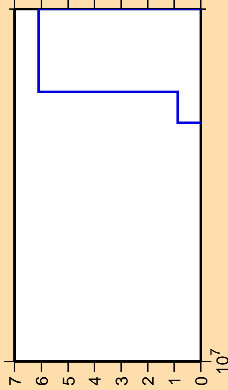
\Delta\sigma/\sigma vs. E for ^{182}\text{Re}(\text{mt117})
