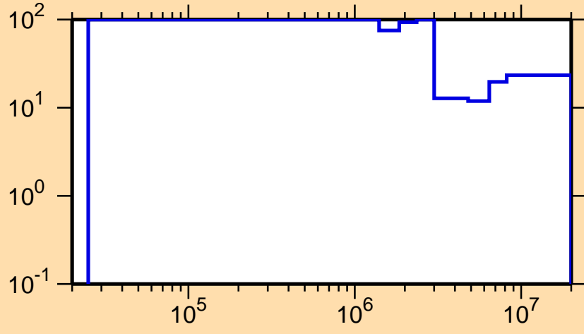
\Delta\sigma/\sigma vs. E for ^{182}\text{Re}(n,n\text{cont.})
