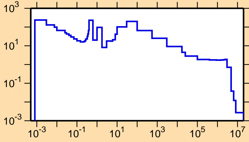
\sigma vs. E for ^{182}\text{Re}(n,\gamma)
