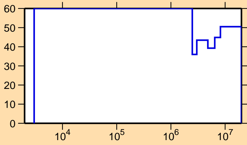
\Delta\sigma/\sigma vs. E for ^{182}\text{Re}(n,n_1)
