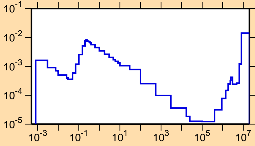
\sigma vs. E for ^{182}\text{Re}(n,p)
