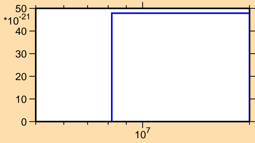
\sigma vs. E for ^{182}\text{Re}(\text{mt } 42)
