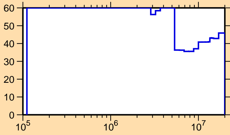
\Delta\sigma/\sigma vs. E for ^{183}\text{Re}(n,n_1)
