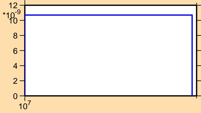
\sigma vs. E for ^{183}\text{Re}(n,2n\alpha)
