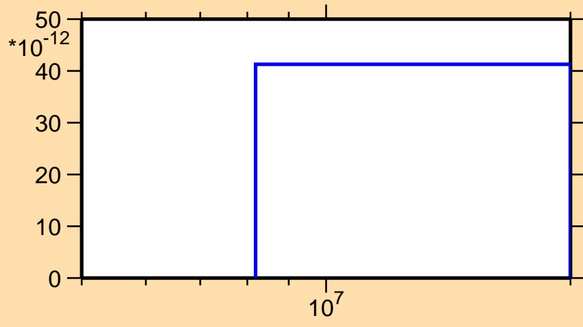
\sigma vs. E for ^{183}\text{Re}(n,\text{He}3)
