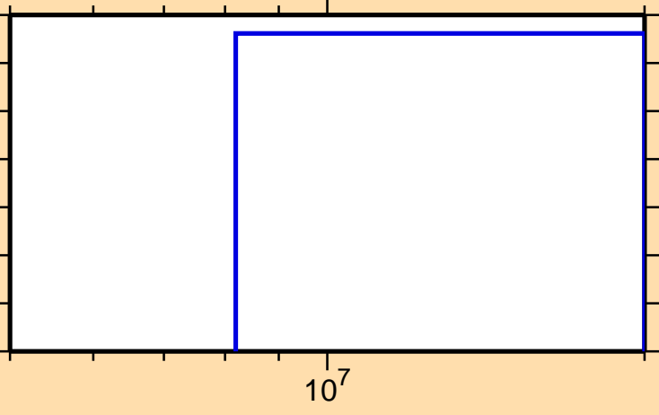
\sigma vs. E for ^{183}\text{Re}(\text{mt } 42)
