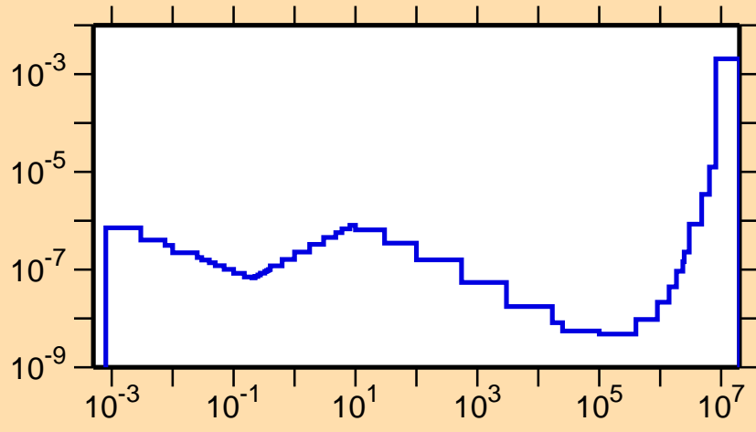
\sigma vs. E for ^{183}\text{Re}(n,\alpha)
