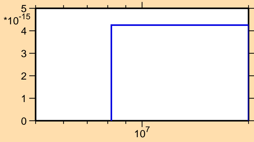
\sigma vs. E for ^{183}\text{Re}(\text{mt117})
