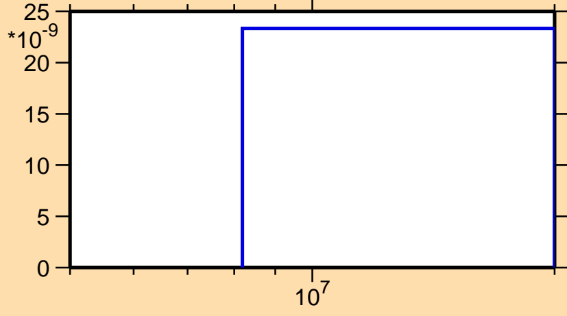
\sigma vs. E for ^{183}\text{Re}(n,\text{nd})
