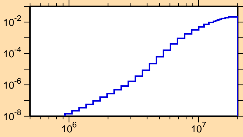
\sigma vs. E for ^{184}\text{Re}(n,p)
