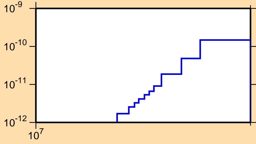
\sigma vs. E for ^{184}\text{Re}(n,p\alpha)
