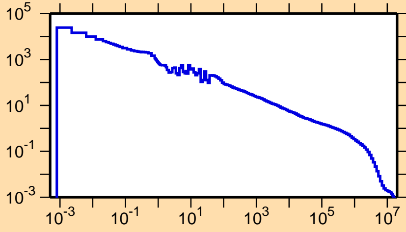
\sigma vs. E for ^{184}\text{Re}(n,\gamma)
