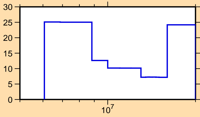
\Delta\sigma/\sigma vs. E for ^{184}\text{Re}(n,2n)
