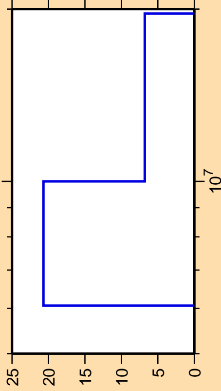
\Delta\sigma/\sigma vs. E for ^{184}\text{Re}(n,2n)
