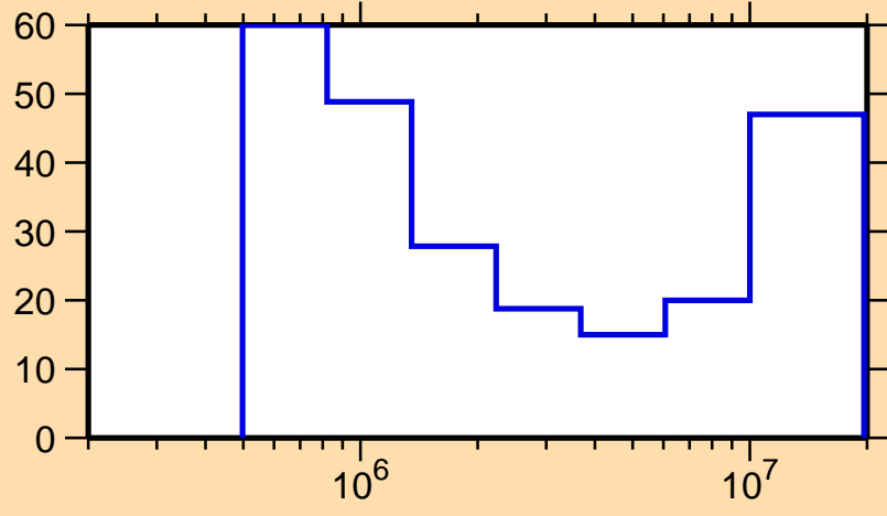
\Delta\sigma/\sigma vs. E for ^{184}\text{Re}(n,n\text{cont.})
