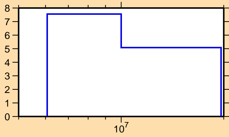
\Delta\sigma/\sigma vs. E for ^{184}\text{Re}(n,\text{nonel.})
