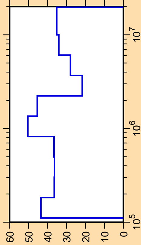
\Delta\sigma/\sigma vs. E for ^{184}\text{Re}(n,n_4)
