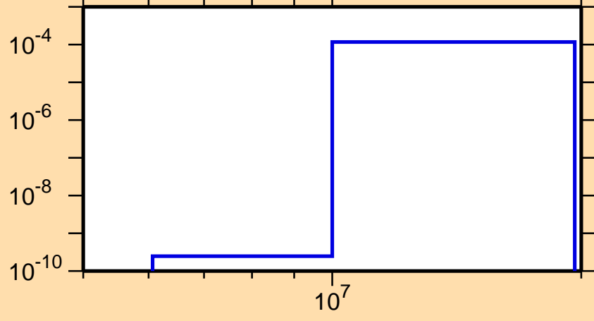
\sigma vs. E for ^{184}\text{Re}(n,t)
